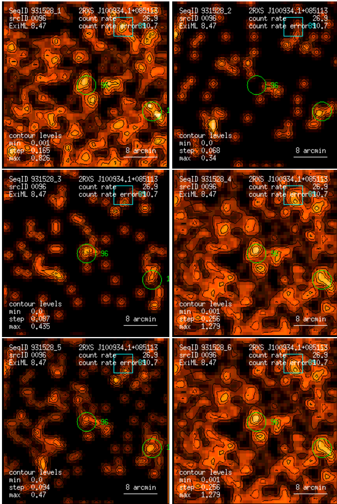
Figure 96: RASS 931528: detection 0096: band rate images, Gaussian filter: (1) PSPC channels 11 – 41, (2) 52 – 90, (3) 91 – 201, (4) 11 – 235, (5) 52 – 201, (6) 11 – 201. Broad band rates in counts/ks. Band rate contour levels in counts/ks/arcmin 2 .
