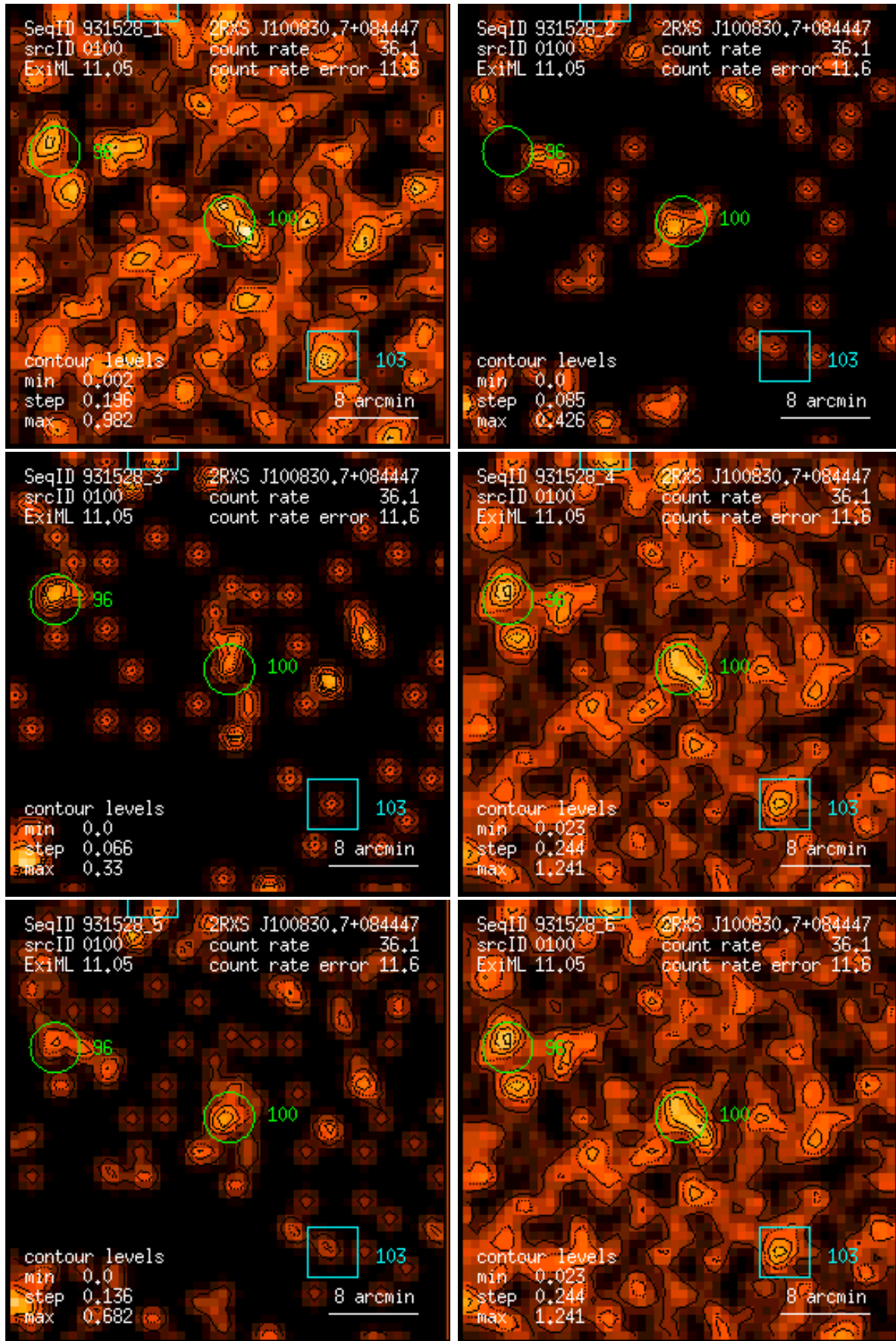
Figure 100: RASS 931528: detection 0100: band rate images, Gaussian filter: (1) PSPC channels 11 – 41, (2) 52 – 90, (3) 91 – 201, (4) 11 – 235, (5) 52 – 201, (6) 11 – 201. Broad band rates in counts/ks. Band rate contour levels in counts/ks/arcmin 2 .
