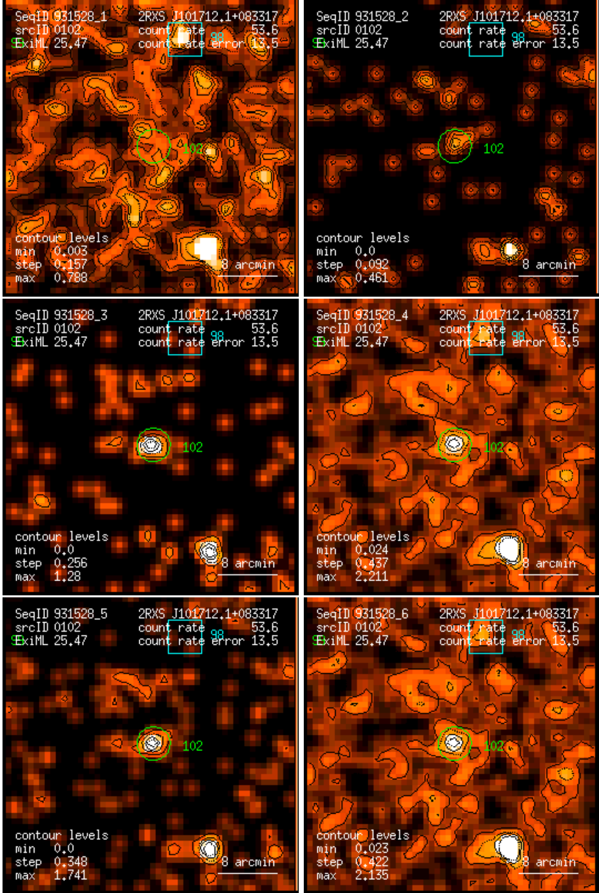
Figure 102: RASS 931528: detection 0102: band rate images, Gaussian filter: (1) PSPC channels 11 – 41, (2) 52 – 90, (3) 91 – 201, (4) 11 – 235, (5) 52 – 201, (6) 11 – 201. Broad band rates in counts/ks. Band rate contour levels in counts/ks/arcmin 2 .
