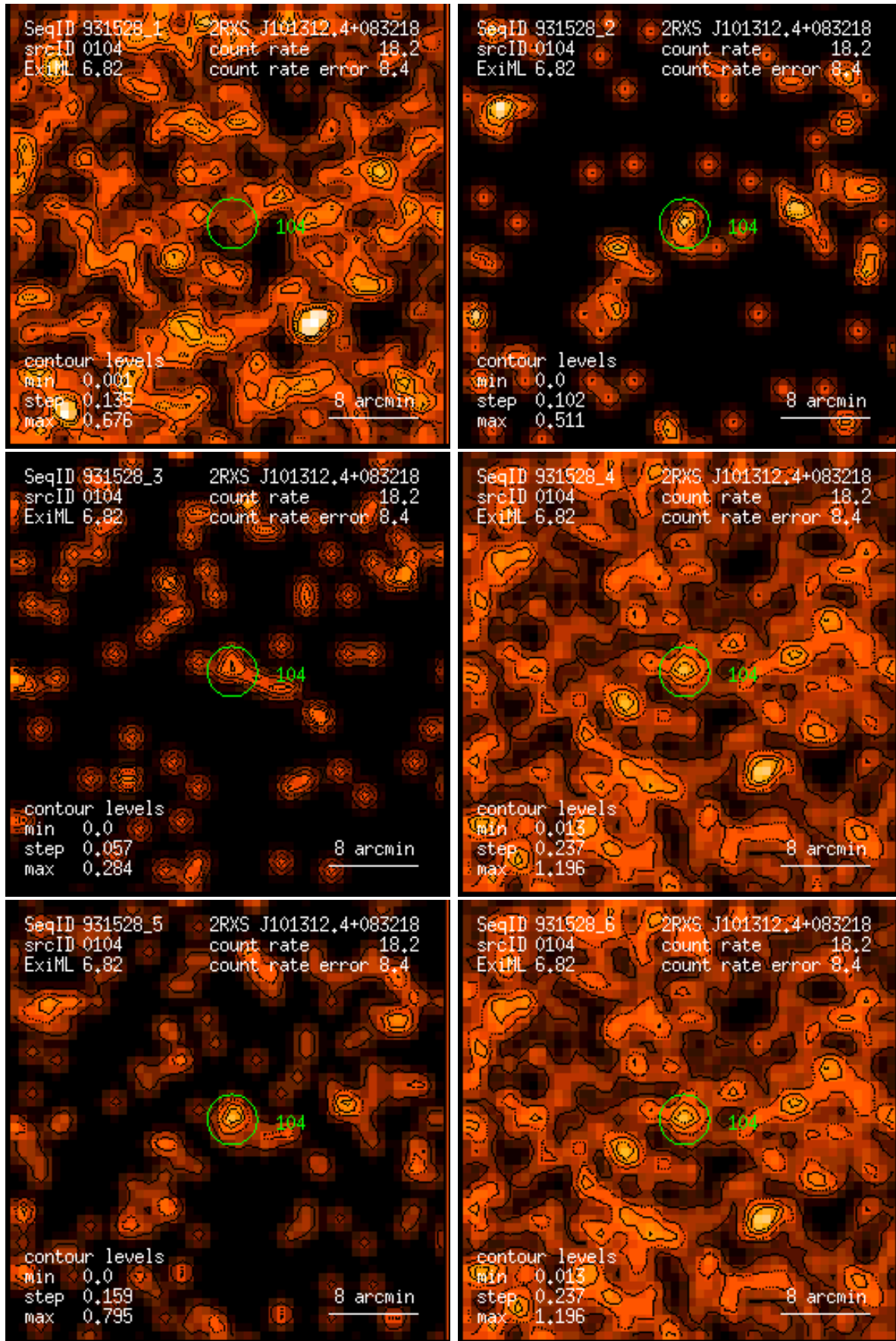
Figure 104: RASS 931528: detection 0104: band rate images, Gaussian filter: (1) PSPC channels 11 – 41, (2) 52 – 90, (3) 91 – 201, (4) 11 – 235, (5) 52 – 201, (6) 11 – 201. Broad band rates in counts/ks. Band rate contour levels in counts/ks/arcmin 2 .
