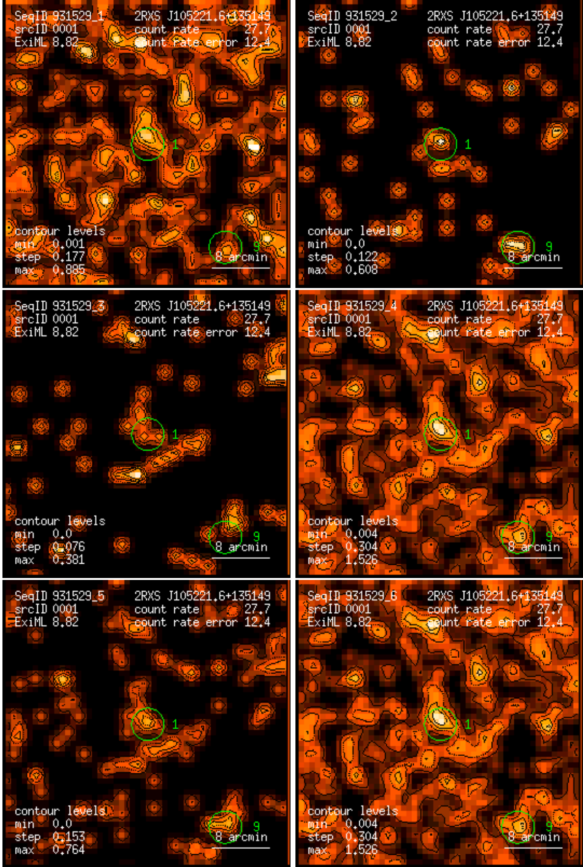
Figure 1: RASS 931529: detection 0001: band rate images, Gaussian filter: (1) PSPC channels 11 – 41, (2) 52 – 90, (3) 91 – 201, (4) 11 – 235, (5) 52 – 201, (6) 11 – 201. Broad band rates in counts/ks. Band rate contour levels in counts/ks/arcmin 2 .
