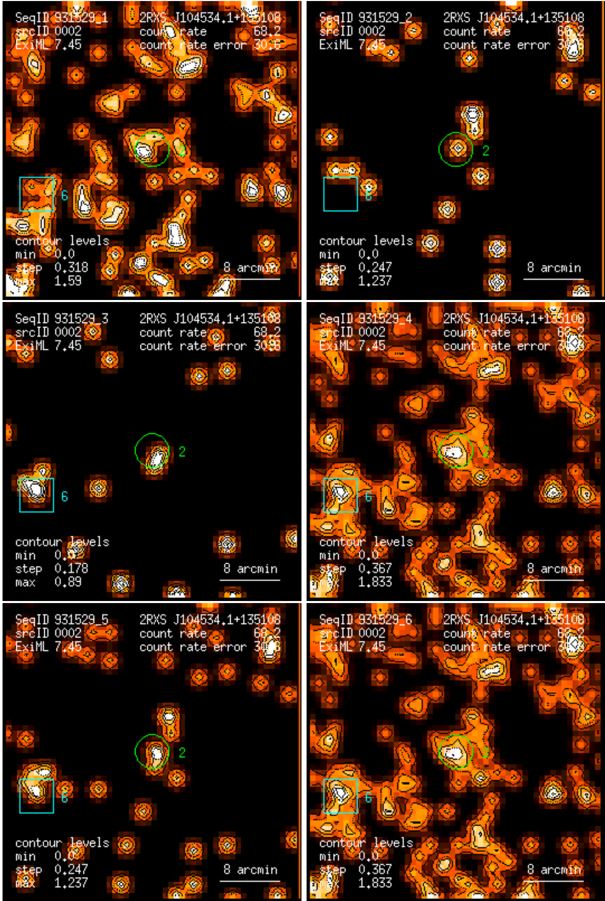
Figure 2: RASS 931529: detection 0002: band rate images, Gaussian filter: (1) PSPC channels 11 – 41, (2) 52 – 90, (3) 91 – 201, (4) 11 – 235, (5) 52 – 201, (6) 11 – 201. Broad band rates in counts/ks. Band rate contour levels in counts/ks/arcmin 2 .
