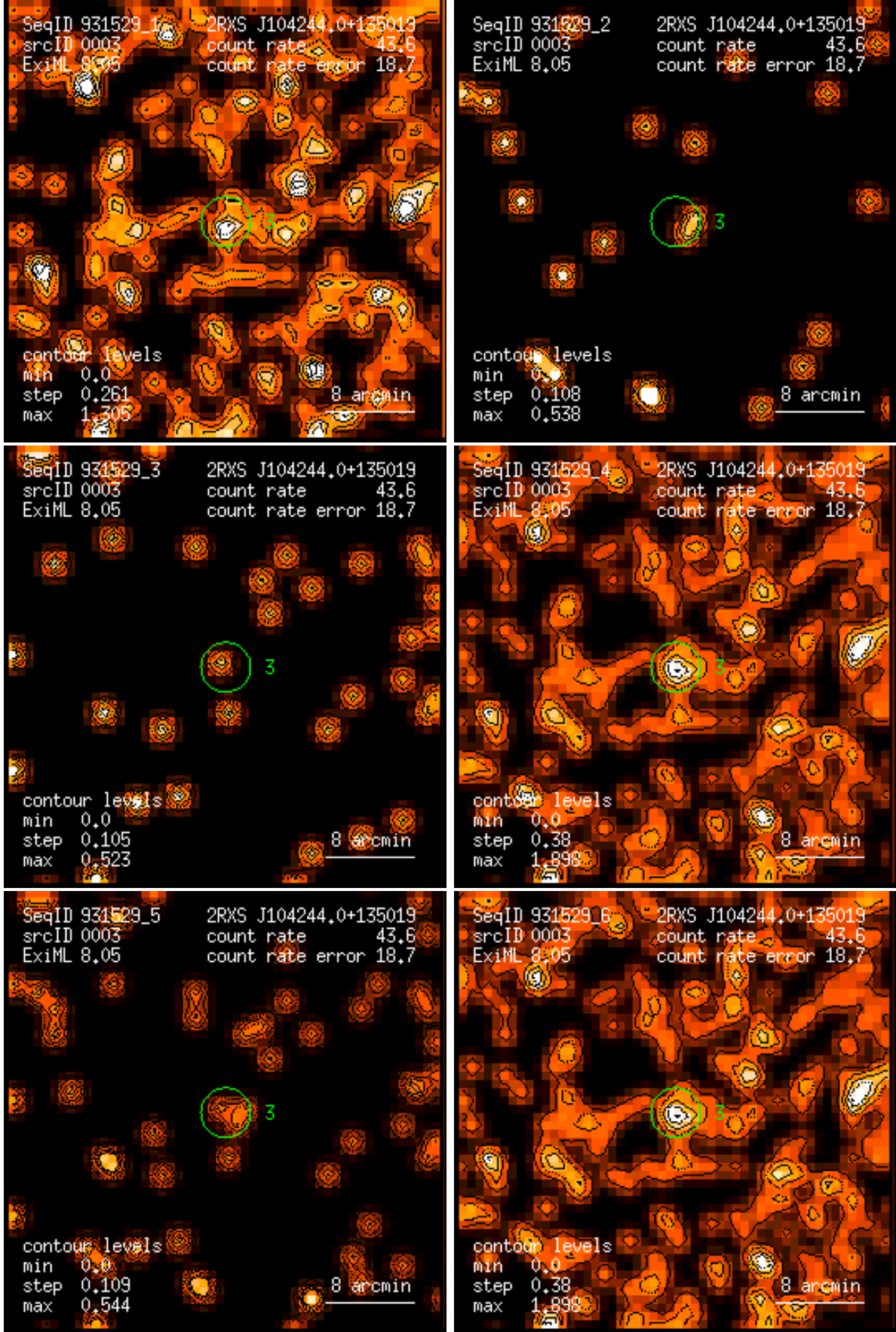
Figure 3: RASS 931529: detection 0003: band rate images, Gaussian filter: (1) PSPC channels 11 – 41, (2) 52 – 90, (3) 91 – 201, (4) 11 – 235, (5) 52 – 201, (6) 11 – 201. Broad band rates in counts/ks. Band rate contour levels in counts/ks/arcmin 2 .
