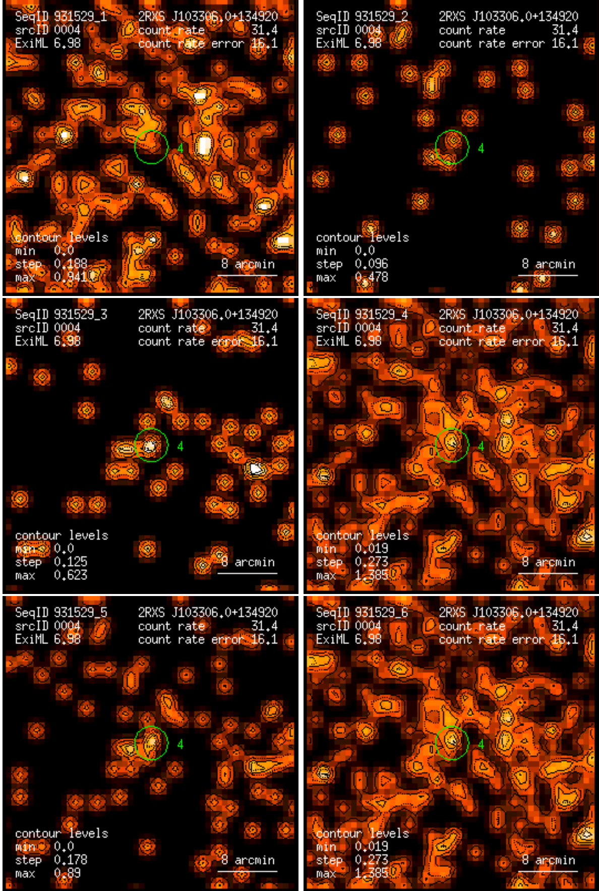
Figure 4: RASS 931529: detection 0004: band rate images, Gaussian filter: (1) PSPC channels 11 – 41, (2) 52 – 90, (3) 91 – 201, (4) 11 – 235, (5) 52 – 201, (6) 11 – 201. Broad band rates in counts/ks. Band rate contour levels in counts/ks/arcmin 2 .
