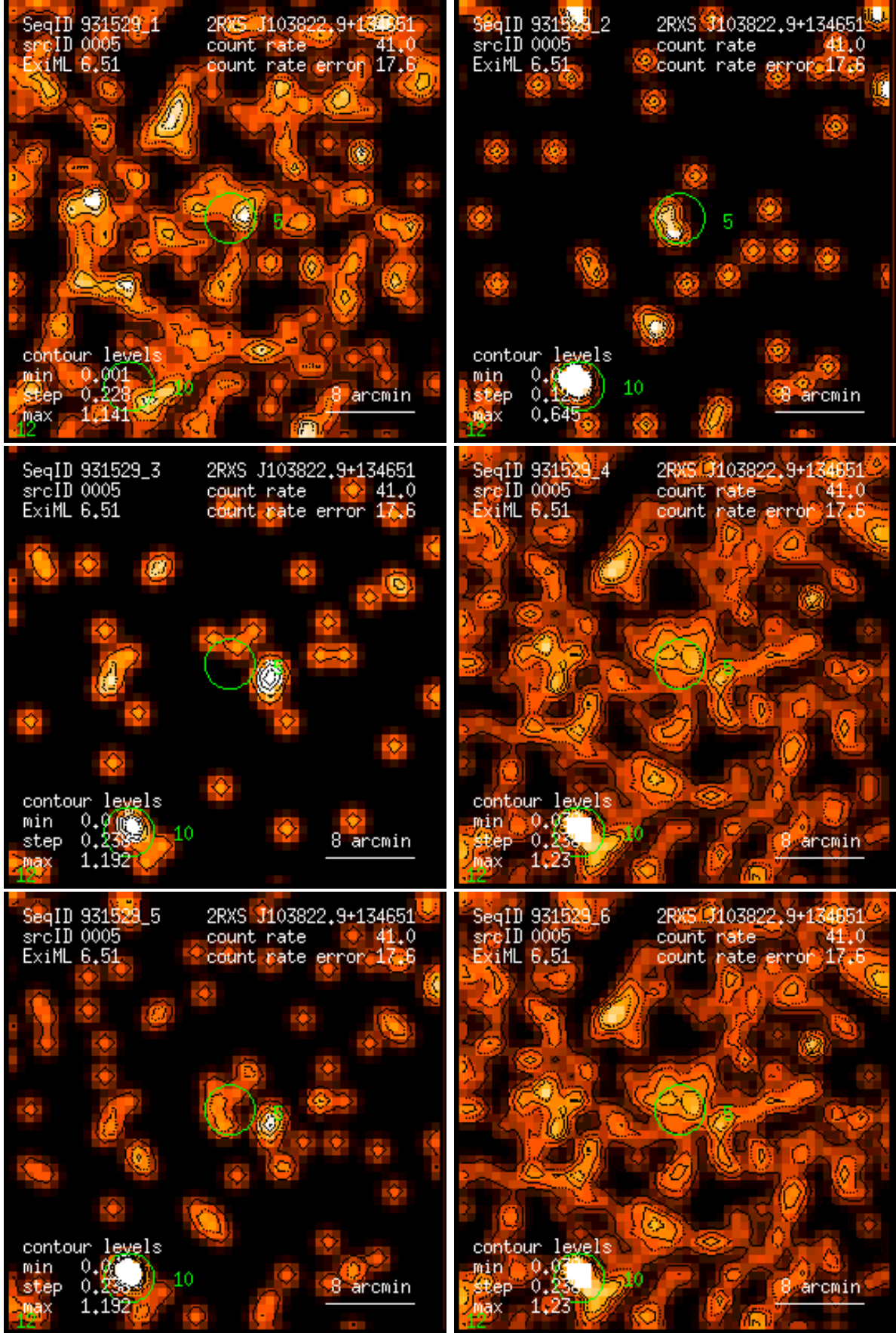
Figure 5: RASS 931529: detection 0005: band rate images, Gaussian filter: (1) PSPC channels 11 – 41, (2) 52 – 90, (3) 91 – 201, (4) 11 – 235, (5) 52 – 201, (6) 11 – 201. Broad band rates in counts/ks. Band rate contour levels in counts/ks/arcmin 2 .
