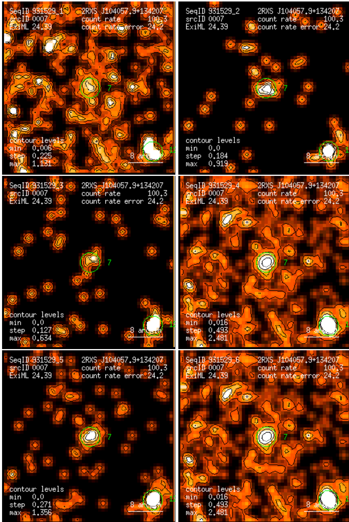
Figure 7: RASS 931529: detection 0007: band rate images, Gaussian filter: (1) PSPC channels 11 – 41, (2) 52 – 90, (3) 91 – 201, (4) 11 – 235, (5) 52 – 201, (6) 11 – 201. Broad band rates in counts/ks. Band rate contour levels in counts/ks/arcmin 2 .
