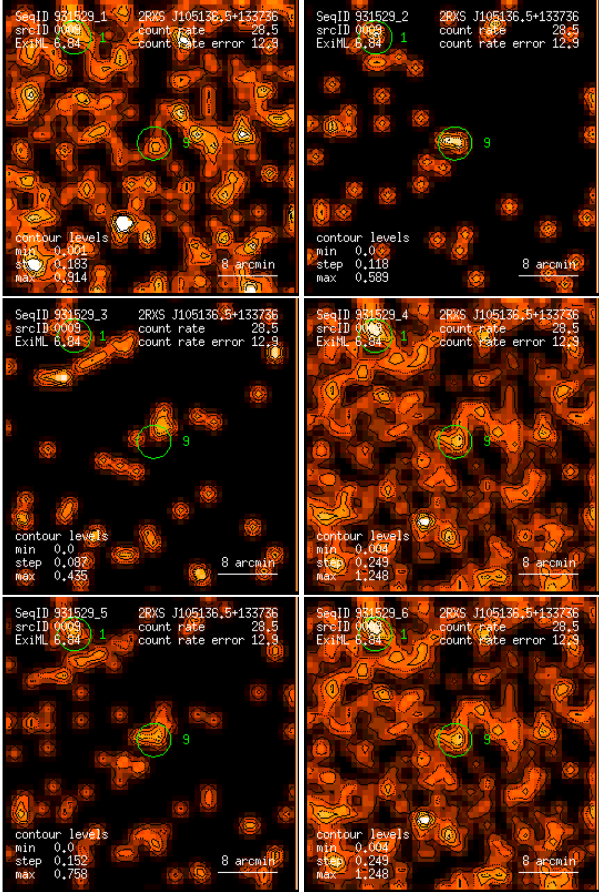
Figure 9: RASS 931529: detection 0009: band rate images, Gaussian filter: (1) PSPC channels 11 – 41, (2) 52 – 90, (3) 91 – 201, (4) 11 – 235, (5) 52 – 201, (6) 11 – 201. Broad band rates in counts/ks. Band rate contour levels in counts/ks/arcmin 2 .
