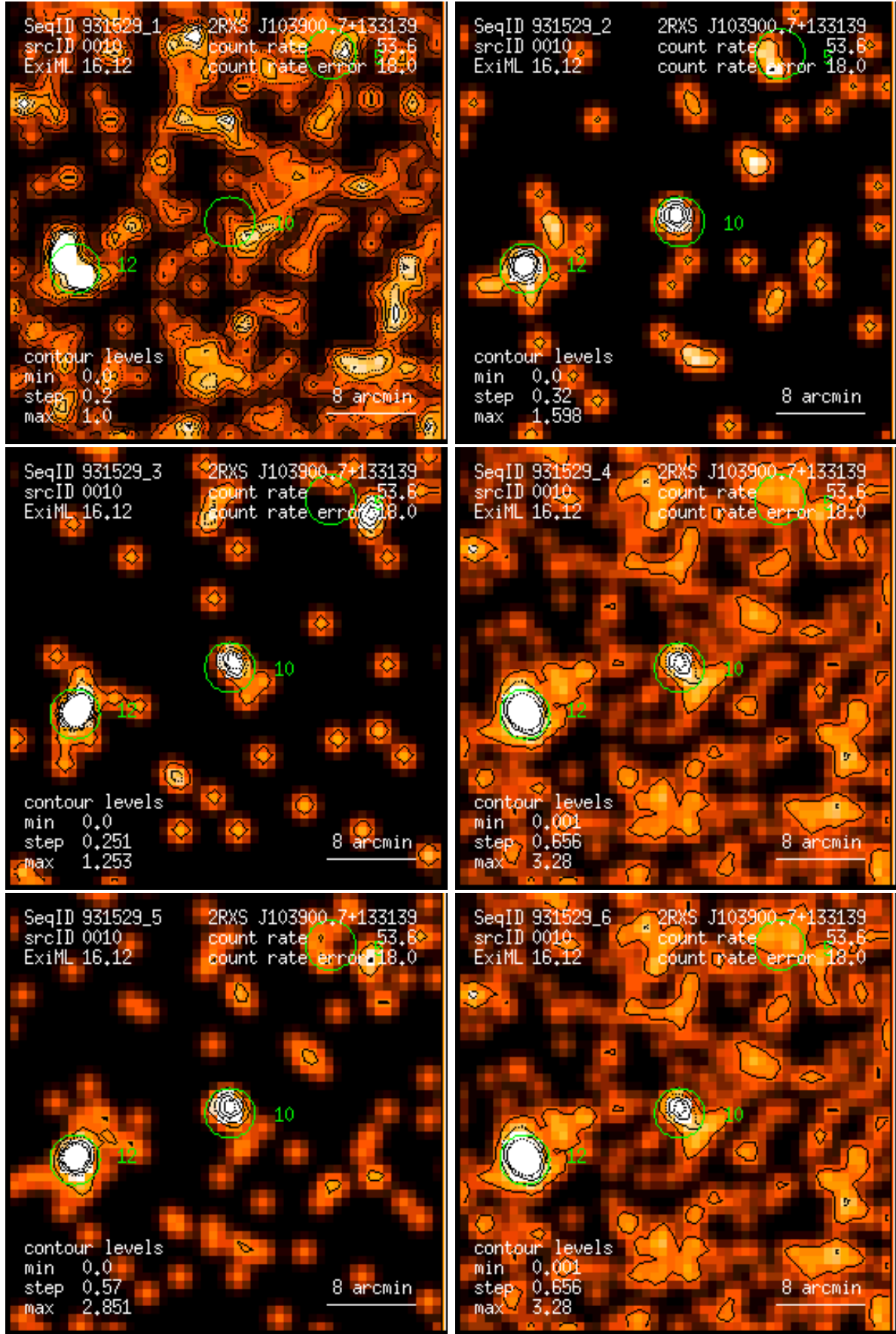
Figure 10: RASS 931529: detection 0010: band rate images, Gaussian filter: (1) PSPC channels 11 – 41, (2) 52 – 90, (3) 91 – 201, (4) 11 – 235, (5) 52 – 201, (6) 11 – 201. Broad band rates in counts/ks. Band rate contour levels in counts/ks/arcmin 2 .
