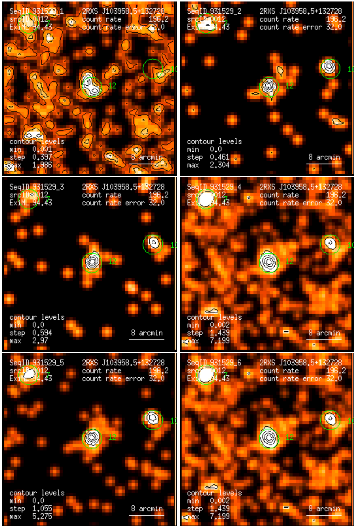
Figure 12: RASS 931529: detection 0012: band rate images, Gaussian filter: (1) PSPC channels 11 – 41, (2) 52 – 90, (3) 91 – 201, (4) 11 – 235, (5) 52 – 201, (6) 11 – 201. Broad band rates in counts/ks. Band rate contour levels in counts/ks/arcmin 2 .
