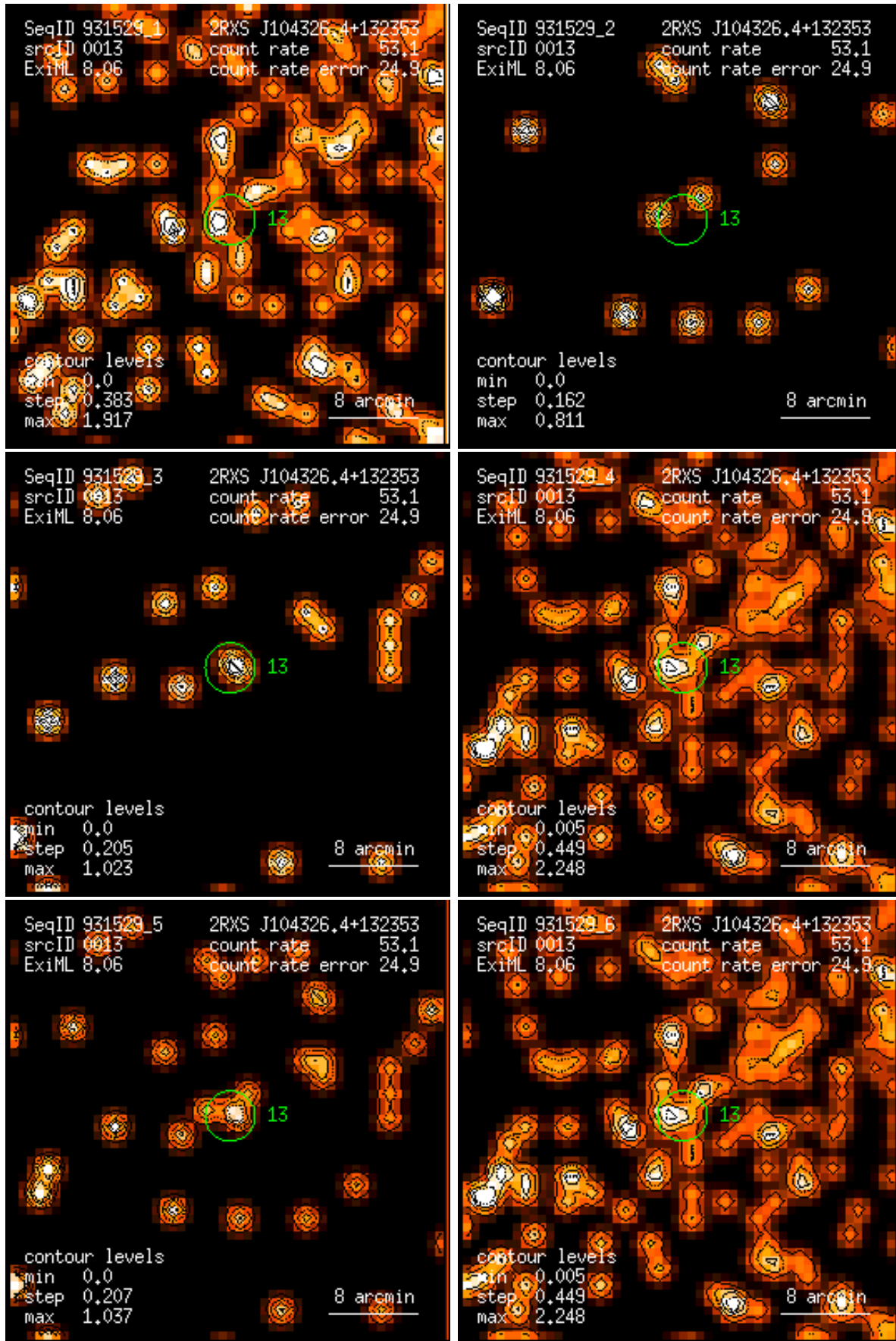
Figure 13: RASS 931529: detection 0013: band rate images, Gaussian filter: (1) PSPC channels 11 – 41, (2) 52 – 90, (3) 91 – 201, (4) 11 – 235, (5) 52 – 201, (6) 11 – 201. Broad band rates in counts/ks. Band rate contour levels in counts/ks/arcmin 2 .
