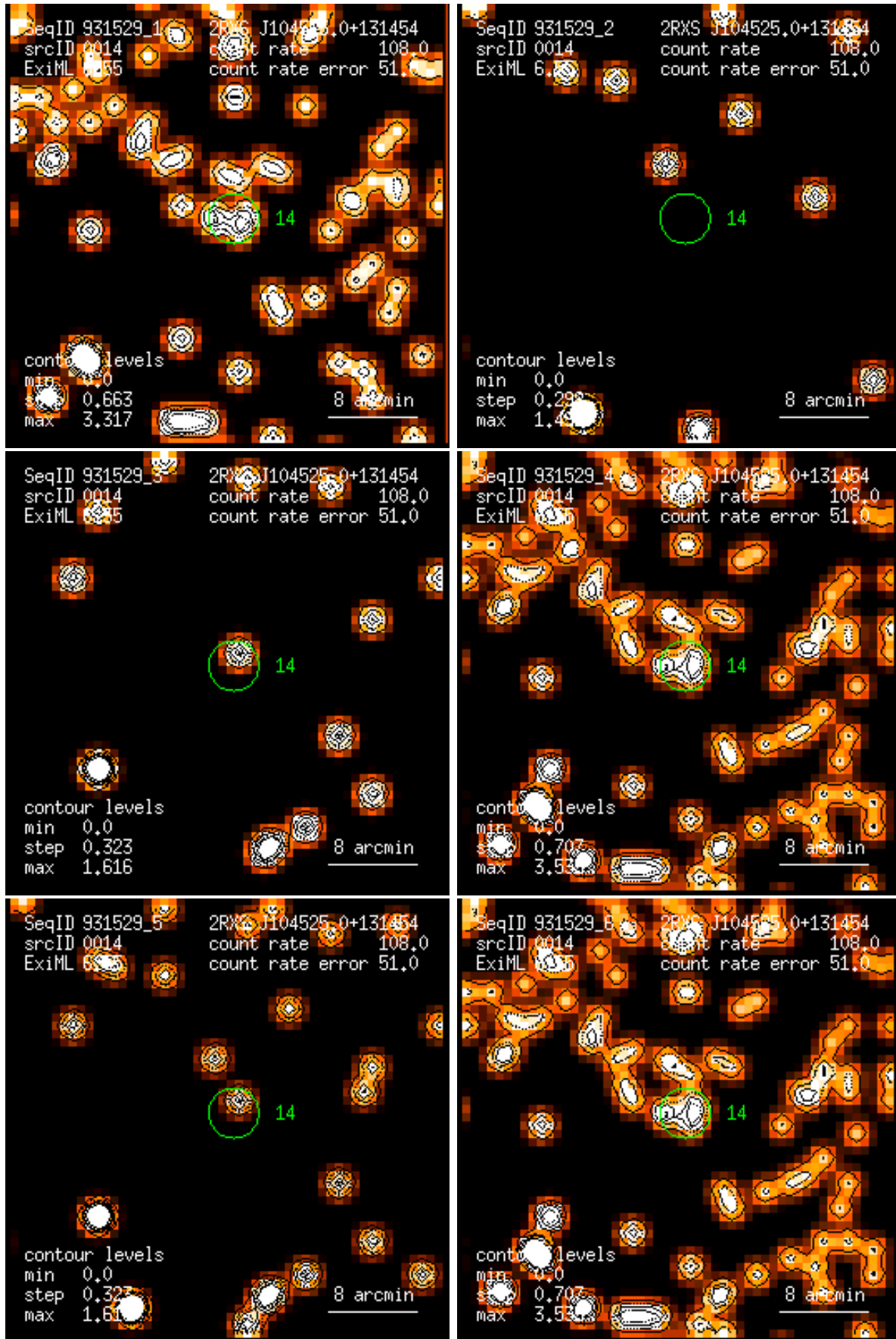
Figure 14: RASS 931529: detection 0014: band rate images, Gaussian filter: (1) PSPC channels 11 – 41, (2) 52 – 90, (3) 91 – 201, (4) 11 – 235, (5) 52 – 201, (6) 11 – 201. Broad band rates in counts/ks. Band rate contour levels in counts/ks/arcmin 2 .
