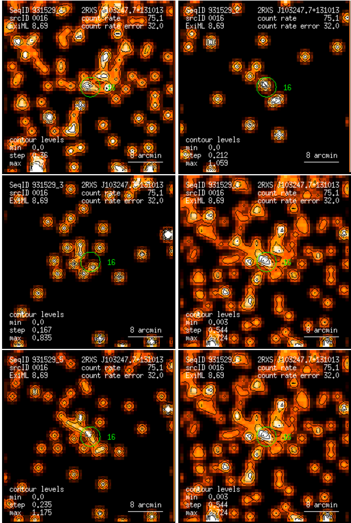
Figure 16: RASS 931529: detection 0016: band rate images, Gaussian filter: (1) PSPC channels 11 – 41, (2) 52 – 90, (3) 91 – 201, (4) 11 – 235, (5) 52 – 201, (6) 11 – 201. Broad band rates in counts/ks. Band rate contour levels in counts/ks/arcmin 2 .
