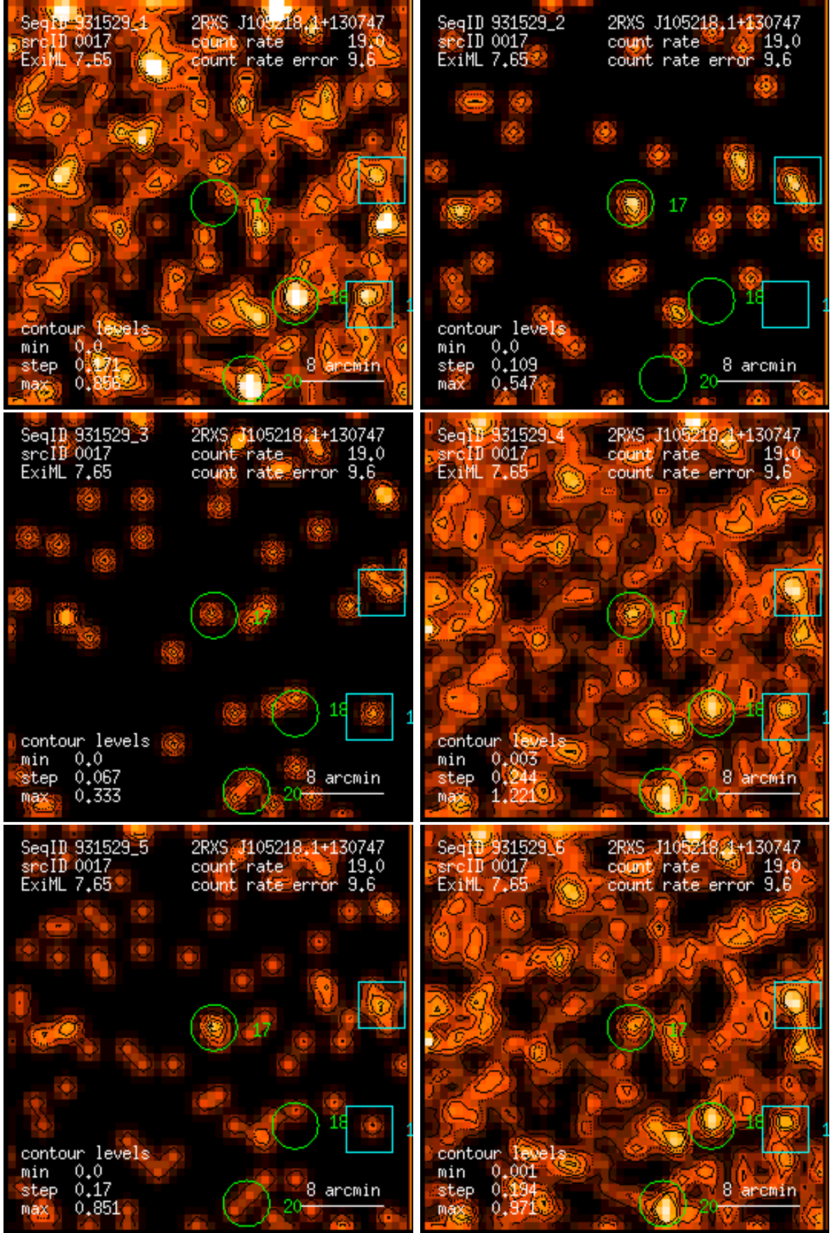
Figure 17: RASS 931529: detection 0017: band rate images, Gaussian filter: (1) PSPC channels 11 – 41, (2) 52 – 90, (3) 91 – 201, (4) 11 – 235, (5) 52 – 201, (6) 11 – 201. Broad band rates in counts/ks. Band rate contour levels in counts/ks/arcmin 2 .
