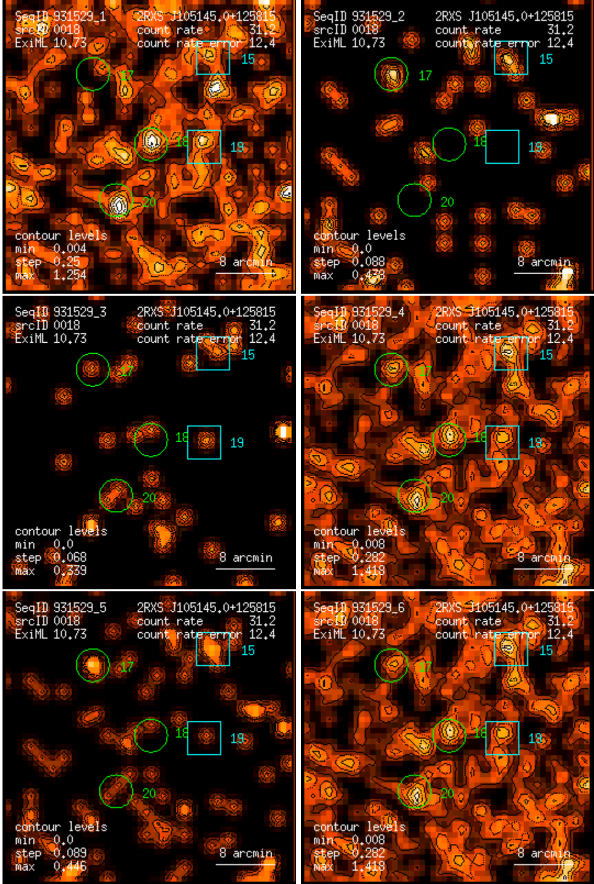
Figure 18: RASS 931529: detection 0018: band rate images, Gaussian filter: (1) PSPC channels 11 – 41, (2) 52 – 90, (3) 91 – 201, (4) 11 – 235, (5) 52 – 201, (6) 11 – 201. Broad band rates in counts/ks. Band rate contour levels in counts/ks/arcmin 2 .
