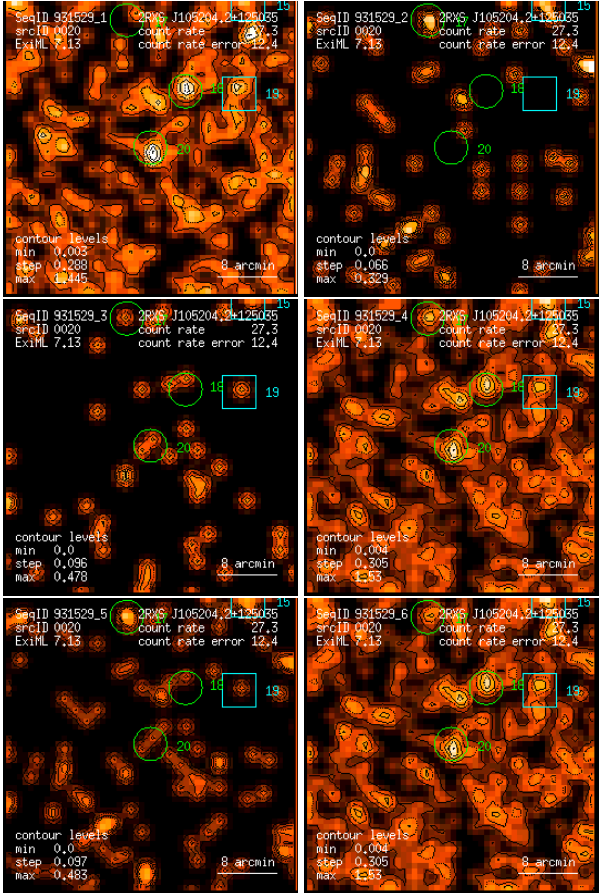
Figure 20: RASS 931529: detection 0020: band rate images, Gaussian filter: (1) PSPC channels 11 – 41, (2) 52 – 90, (3) 91 – 201, (4) 11 – 235, (5) 52 – 201, (6) 11 – 201. Broad band rates in counts/ks. Band rate contour levels in counts/ks/arcmin 2 .
