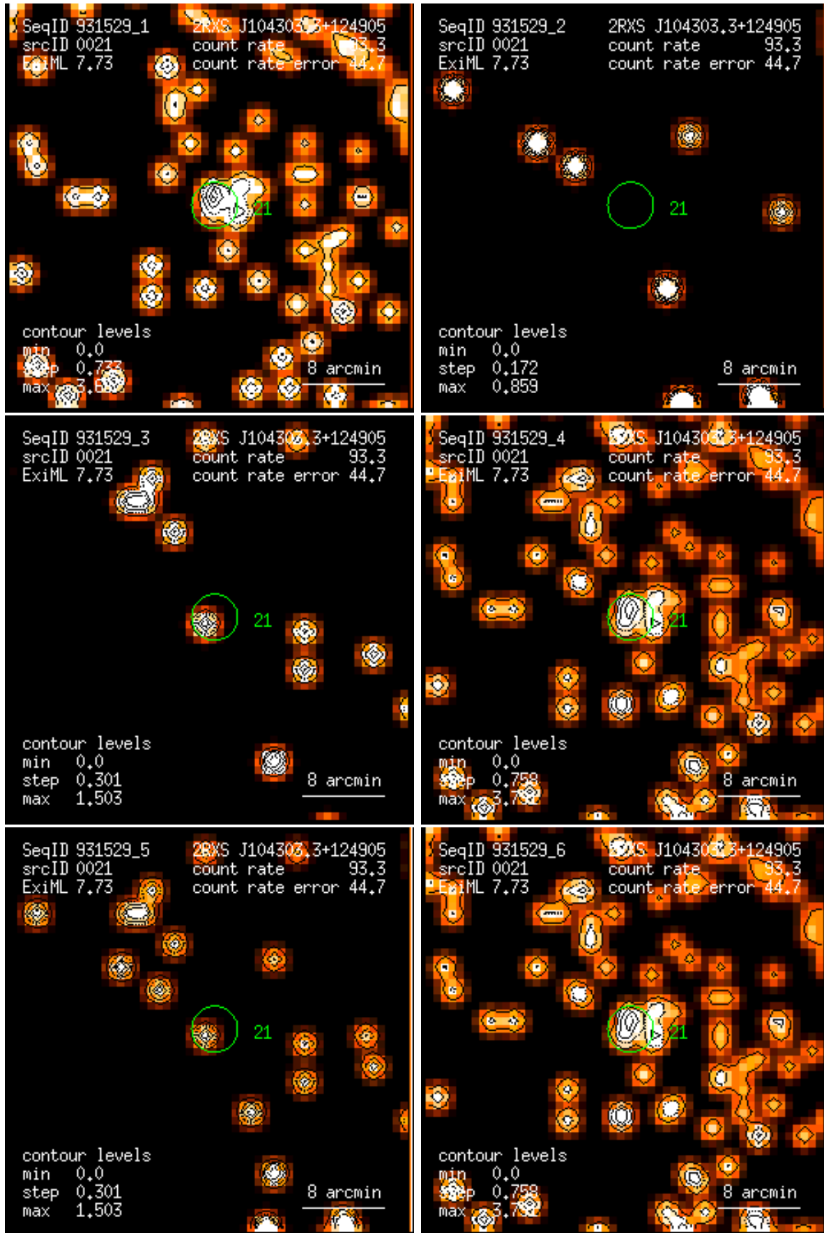
Figure 21: RASS 931529: detection 0021: band rate images, Gaussian filter: (1) PSPC channels 11 – 41, (2) 52 – 90, (3) 91 – 201, (4) 11 – 235, (5) 52 – 201, (6) 11 – 201. Broad band rates in counts/ks. Band rate contour levels in counts/ks/arcmin 2 .
