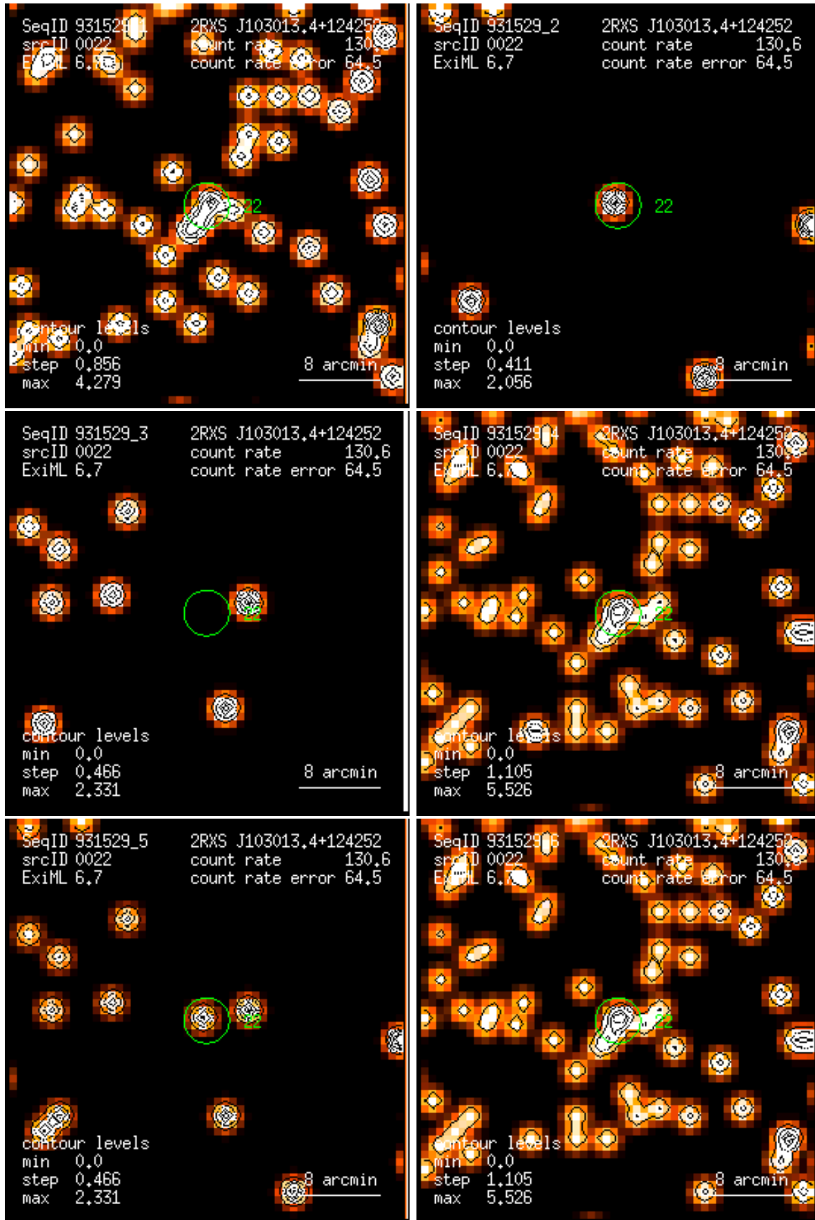
Figure 22: RASS 931529: detection 0022: band rate images, Gaussian filter: (1) PSPC channels 11 – 41, (2) 52 – 90, (3) 91 – 201, (4) 11 – 235, (5) 52 – 201, (6) 11 – 201. Broad band rates in counts/ks. Band rate contour levels in counts/ks/arcmin 2 .
