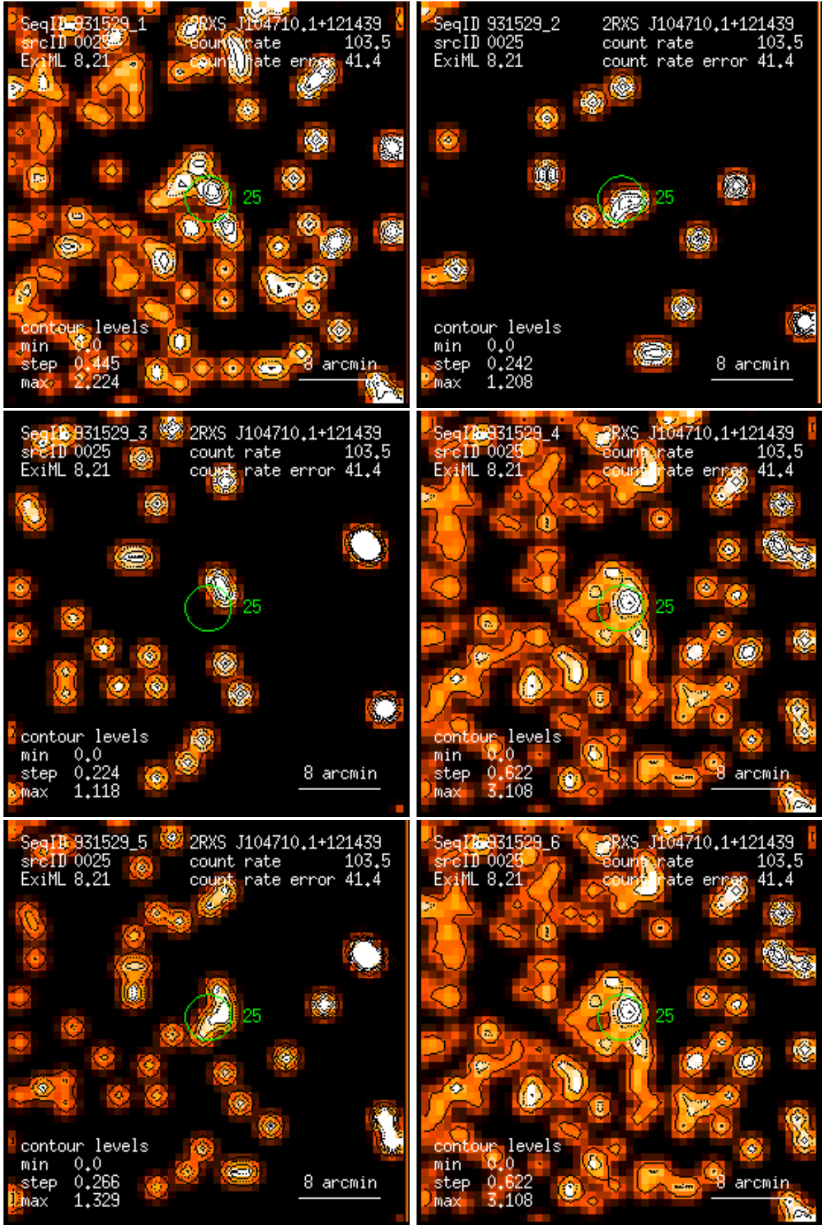
Figure 25: RASS 931529: detection 0025: band rate images, Gaussian filter: (1) PSPC channels 11 – 41, (2) 52 – 90, (3) 91 – 201, (4) 11 – 235, (5) 52 – 201, (6) 11 – 201. Broad band rates in counts/ks. Band rate contour levels in counts/ks/arcmin 2 .
