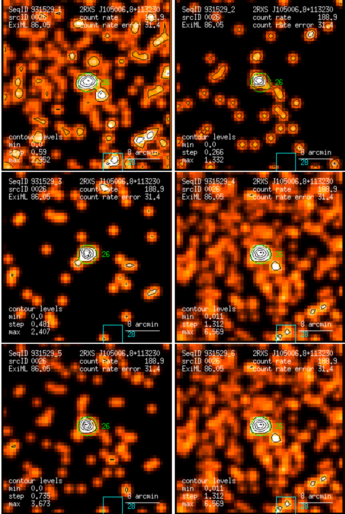
Figure 26: RASS 931529: detection 0026: band rate images, Gaussian filter: (1) PSPC channels 11 – 41, (2) 52 – 90, (3) 91 – 201, (4) 11 – 235, (5) 52 – 201, (6) 11 – 201. Broad band rates in counts/ks. Band rate contour levels in counts/ks/arcmin 2 .
