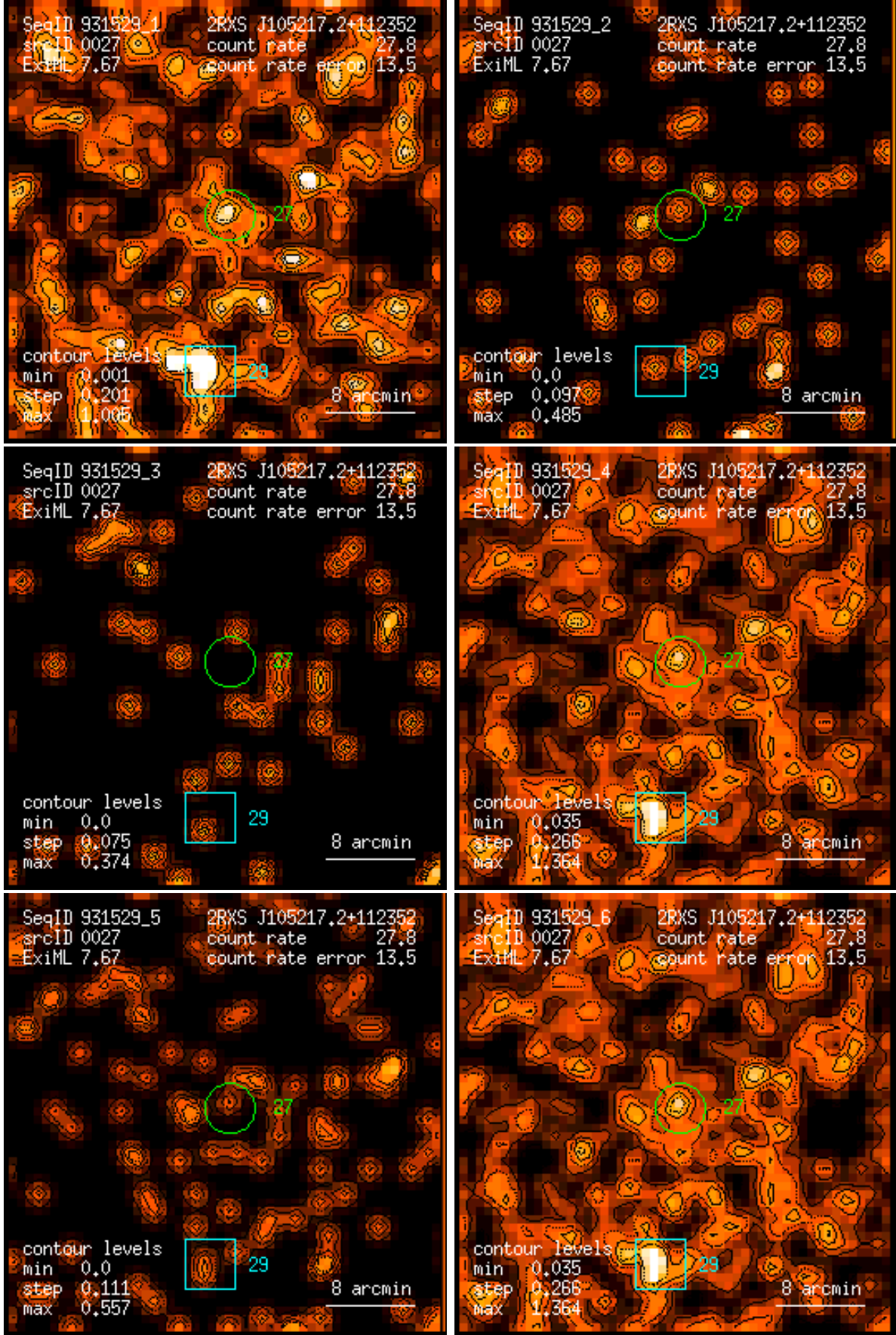
Figure 27: RASS 931529: detection 0027: band rate images, Gaussian filter: (1) PSPC channels 11 – 41, (2) 52 – 90, (3) 91 – 201, (4) 11 – 235, (5) 52 – 201, (6) 11 – 201. Broad band rates in counts/ks. Band rate contour levels in counts/ks/arcmin 2 .
