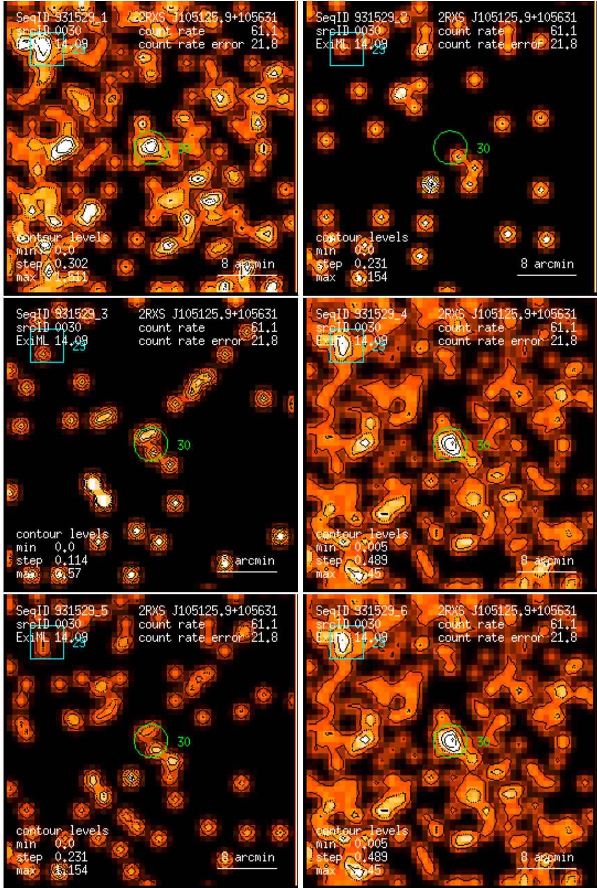
Figure 30: RASS 931529: detection 0030: band rate images, Gaussian filter: (1) PSPC channels 11 – 41, (2) 52 – 90, (3) 91 – 201, (4) 11 – 235, (5) 52 – 201, (6) 11 – 201. Broad band rates in counts/ks. Band rate contour levels in counts/ks/arcmin 2 .
