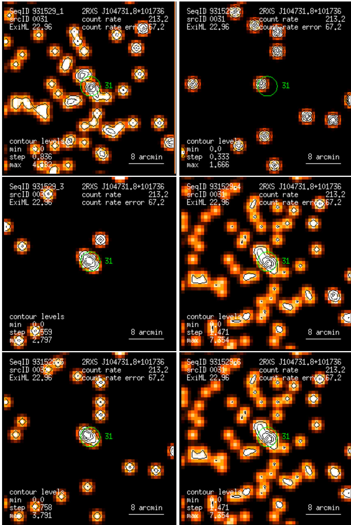
Figure 31: RASS 931529: detection 0031: band rate images, Gaussian filter: (1) PSPC channels 11 – 41, (2) 52 – 90, (3) 91 – 201, (4) 11 – 235, (5) 52 – 201, (6) 11 – 201. Broad band rates in counts/ks. Band rate contour levels in counts/ks/arcmin 2 .
