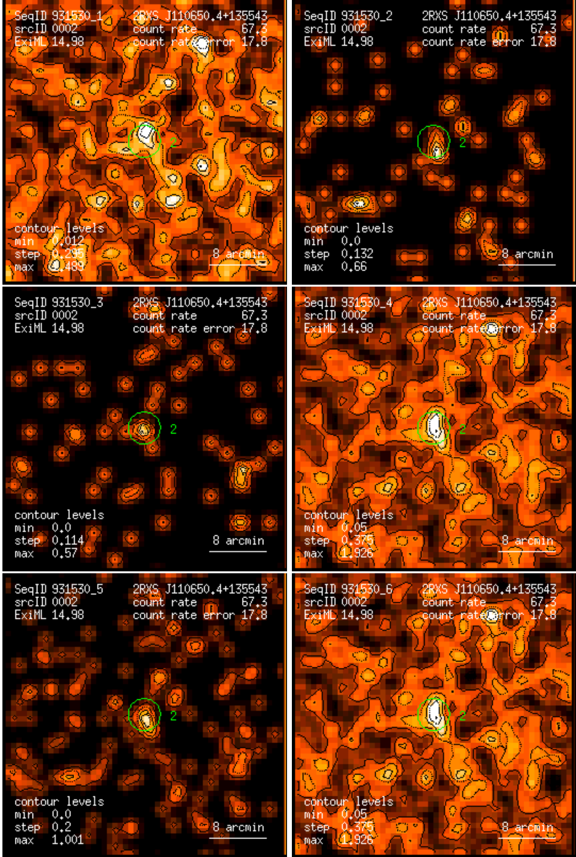
Figure 2: RASS 931530: detection 0002: band rate images, Gaussian filter: (1) PSPC channels 11 – 41, (2) 52 – 90, (3) 91 – 201, (4) 11 – 235, (5) 52 – 201, (6) 11 – 201. Broad band rates in counts/ks. Band rate contour levels in counts/ks/arcmin 2 .
