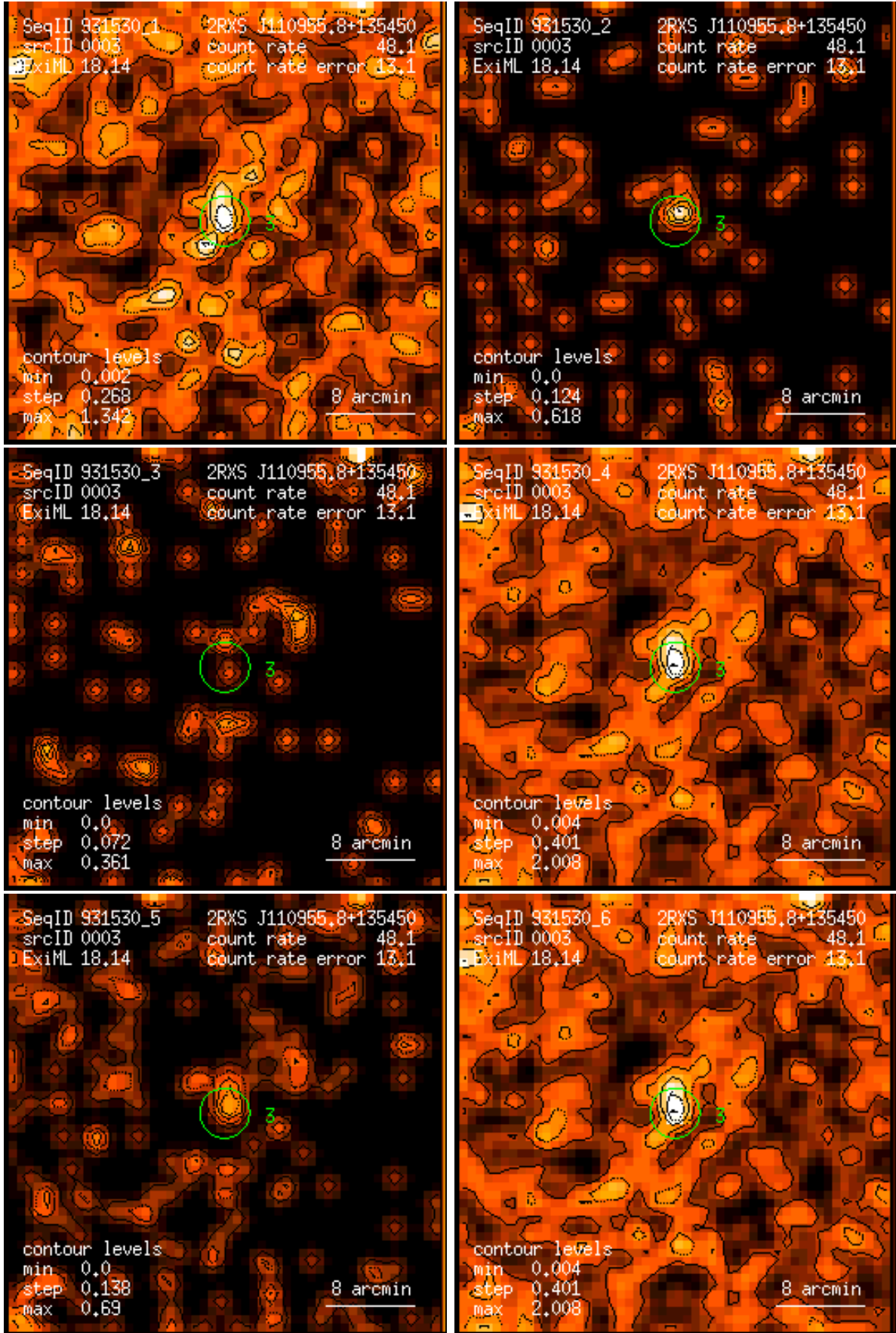
Figure 3: RASS 931530: detection 0003: band rate images, Gaussian filter: (1) PSPC channels 11 – 41, (2) 52 – 90, (3) 91 – 201, (4) 11 – 235, (5) 52 – 201, (6) 11 – 201. Broad band rates in counts/ks. Band rate contour levels in counts/ks/arcmin 2 .
