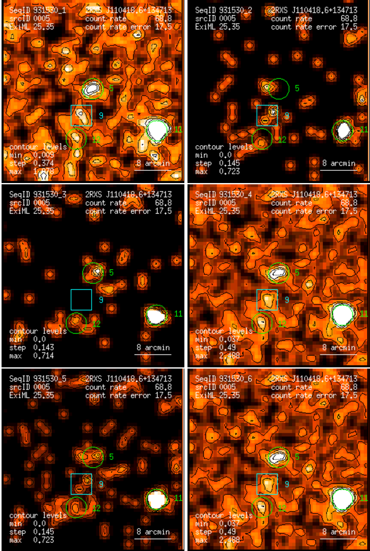
Figure 5: RASS 931530: detection 0005: band rate images, Gaussian filter: (1) PSPC channels 11 – 41, (2) 52 – 90, (3) 91 – 201, (4) 11 – 235, (5) 52 – 201, (6) 11 – 201. Broad band rates in counts/ks. Band rate contour levels in counts/ks/arcmin 2 .
