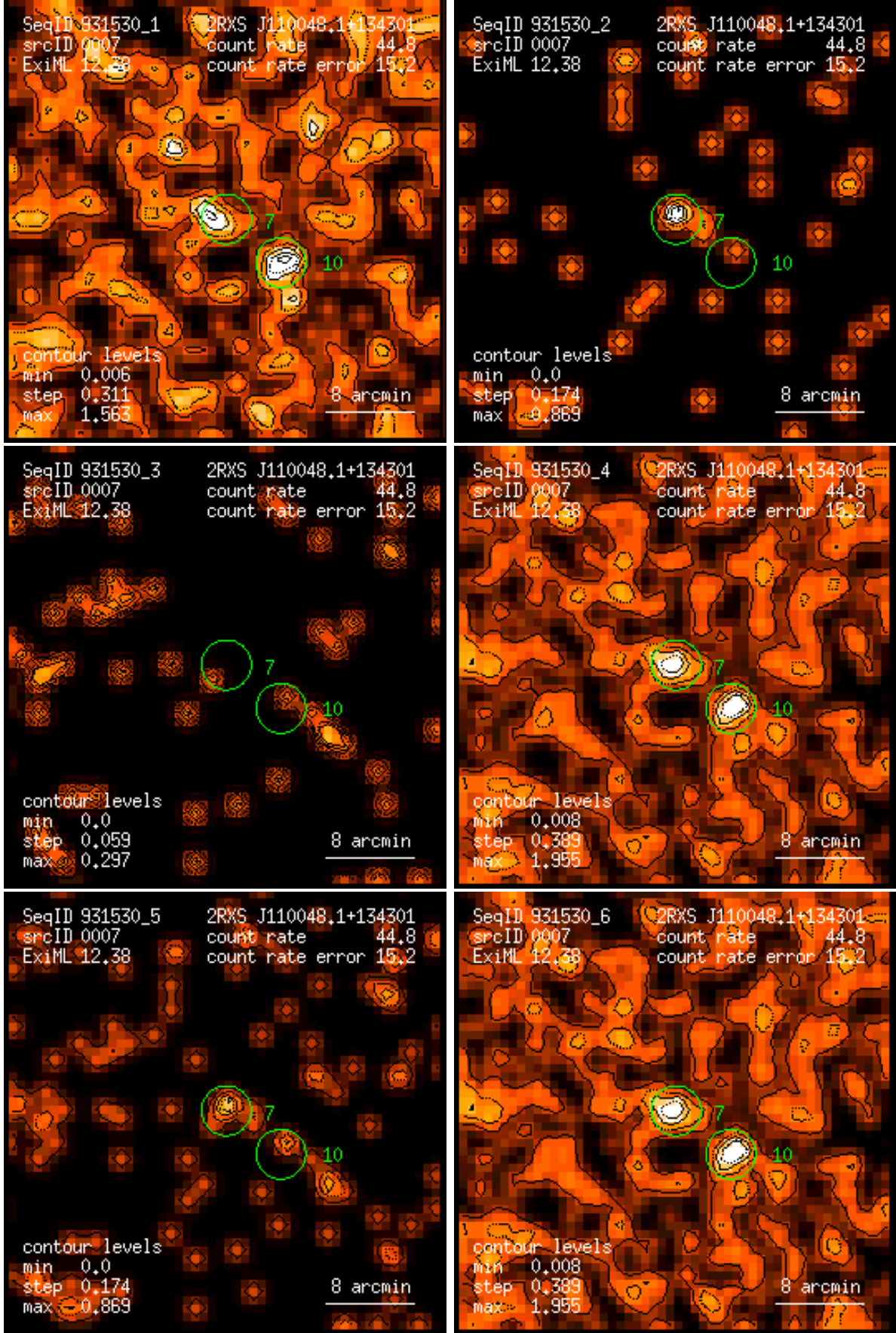
Figure 7: RASS 931530: detection 0007: band rate images, Gaussian filter: (1) PSPC channels 11 – 41, (2) 52 – 90, (3) 91 – 201, (4) 11 – 235, (5) 52 – 201, (6) 11 – 201. Broad band rates in counts/ks. Band rate contour levels in counts/ks/arcmin 2 .
