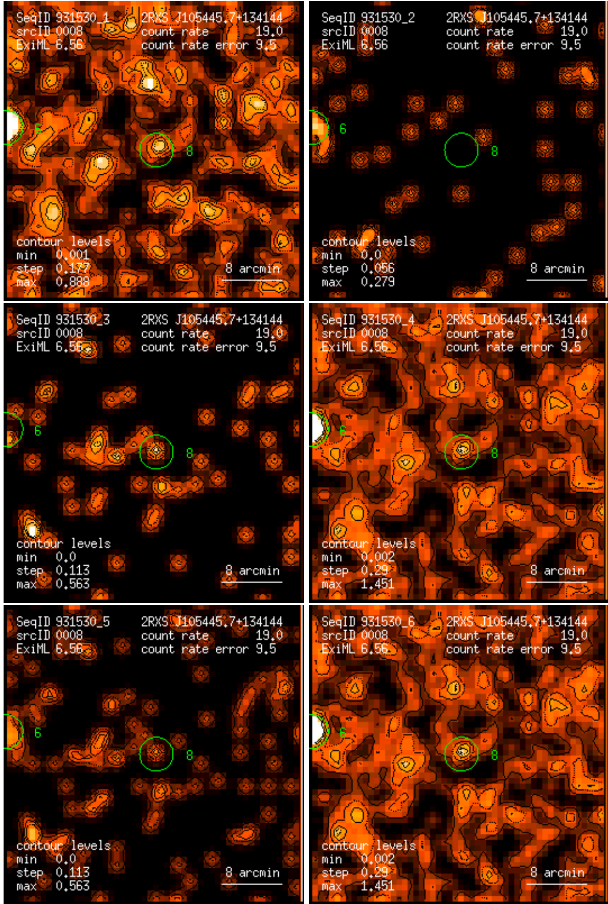
Figure 8: RASS 931530: detection 0008: band rate images, Gaussian filter: (1) PSPC channels 11 – 41, (2) 52 – 90, (3) 91 – 201, (4) 11 – 235, (5) 52 – 201, (6) 11 – 201. Broad band rates in counts/ks. Band rate contour levels in counts/ks/arcmin 2 .
