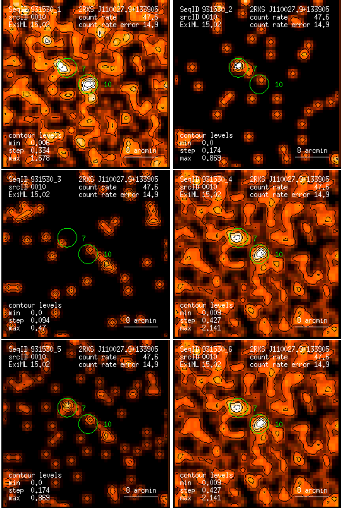
Figure 10: RASS 931530: detection 0010: band rate images, Gaussian filter: (1) PSPC channels 11 – 41, (2) 52 – 90, (3) 91 – 201, (4) 11 – 235, (5) 52 – 201, (6) 11 – 201. Broad band rates in counts/ks. Band rate contour levels in counts/ks/arcmin 2 .
