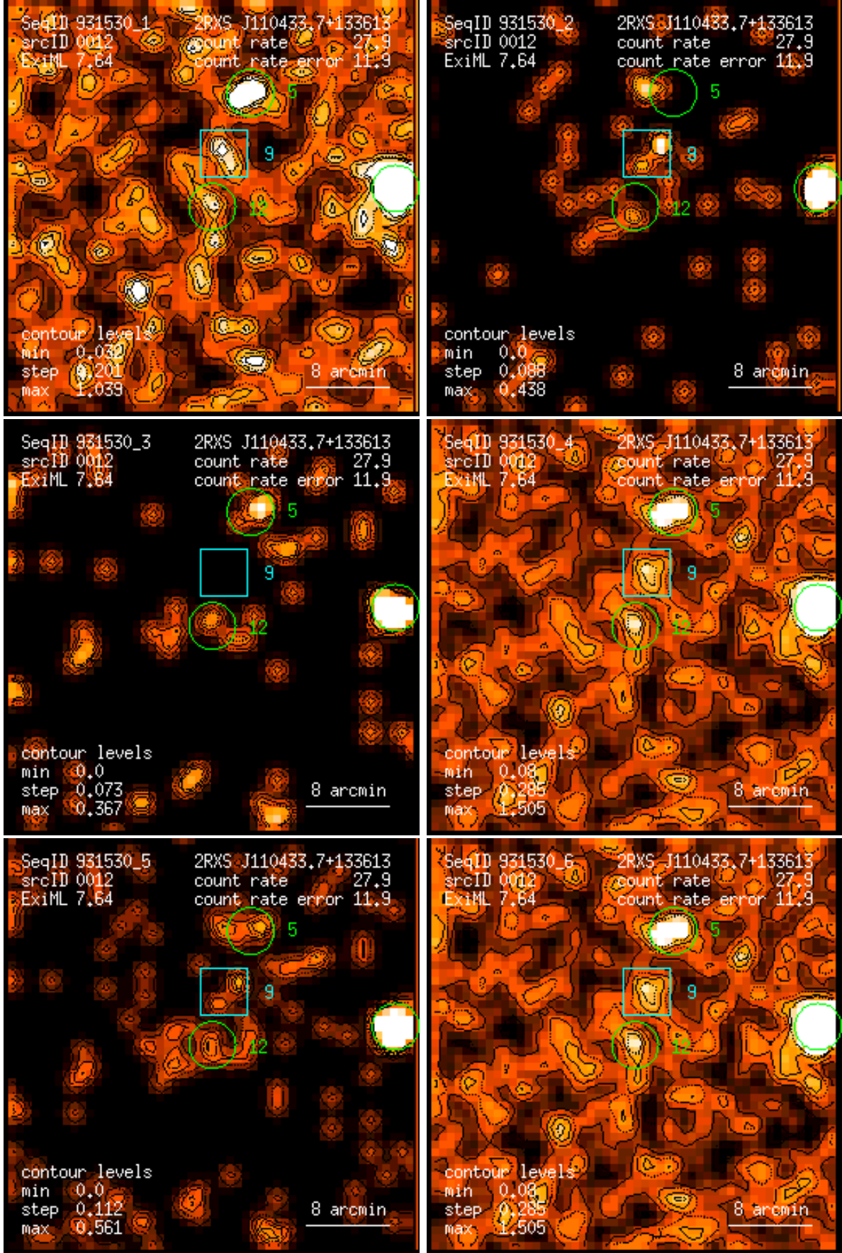
Figure 12: RASS 931530: detection 0012: band rate images, Gaussian filter: (1) PSPC channels 11 – 41, (2) 52 – 90, (3) 91 – 201, (4) 11 – 235, (5) 52 – 201, (6) 11 – 201. Broad band rates in counts/ks. Band rate contour levels in counts/ks/arcmin 2 .
