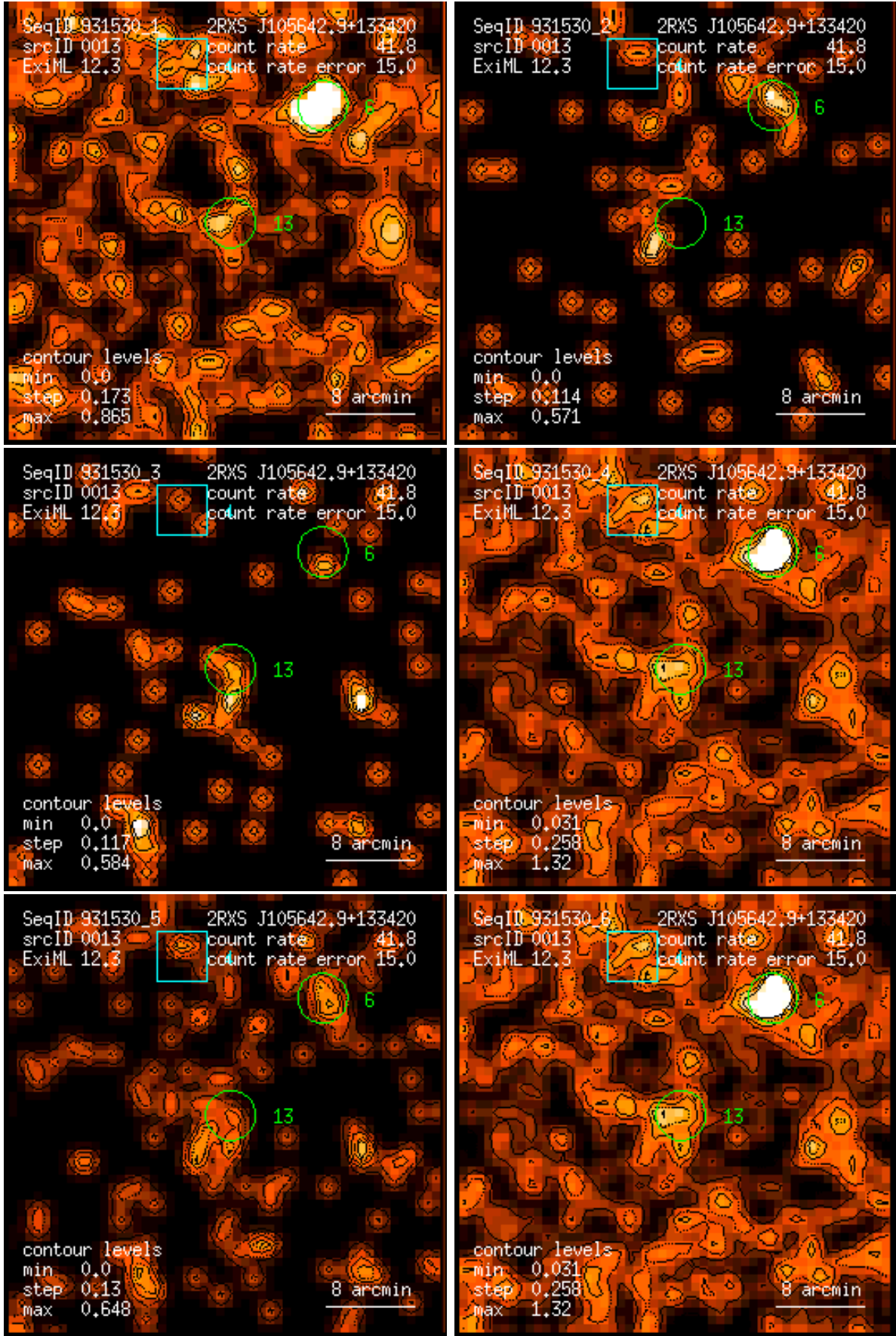
Figure 13: RASS 931530: detection 0013: band rate images, Gaussian filter: (1) PSPC channels 11 – 41, (2) 52 – 90, (3) 91 – 201, (4) 11 – 235, (5) 52 – 201, (6) 11 – 201. Broad band rates in counts/ks. Band rate contour levels in counts/ks/arcmin 2 .
