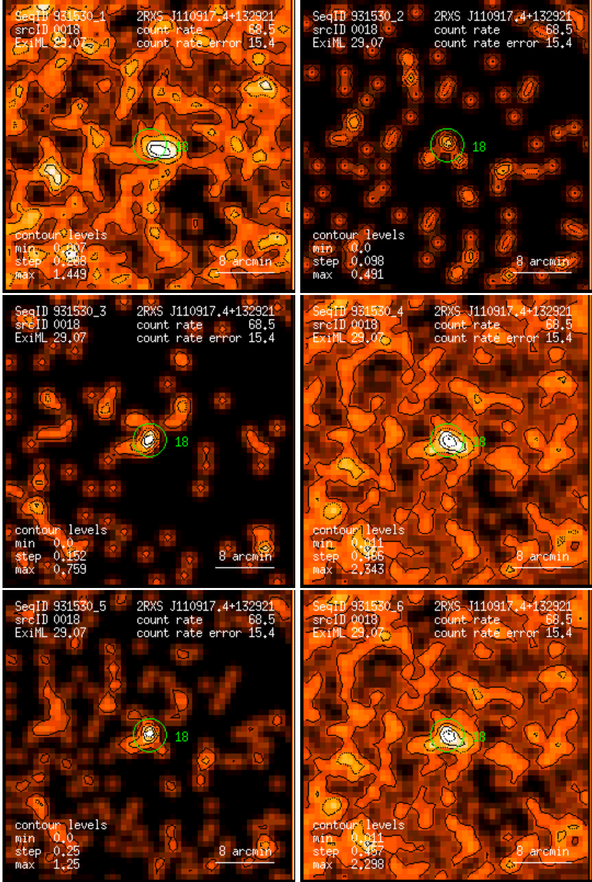
Figure 18: RASS 931530: detection 0018: band rate images, Gaussian filter: (1) PSPC channels 11 – 41, (2) 52 – 90, (3) 91 – 201, (4) 11 – 235, (5) 52 – 201, (6) 11 – 201. Broad band rates in counts/ks. Band rate contour levels in counts/ks/arcmin 2 .
