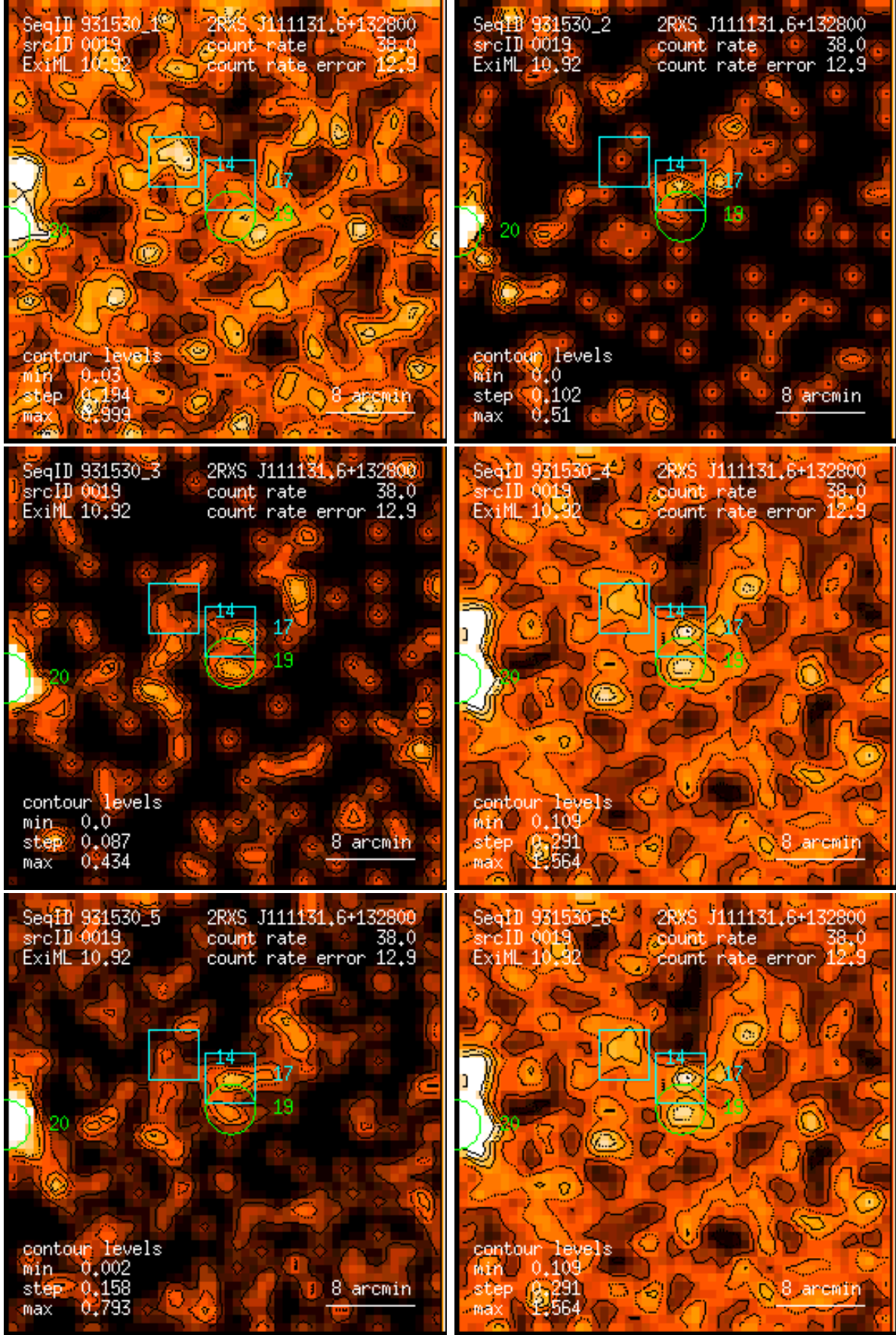
Figure 19: RASS 931530: detection 0019: band rate images, Gaussian filter: (1) PSPC channels 11 – 41, (2) 52 – 90, (3) 91 – 201, (4) 11 – 235, (5) 52 – 201, (6) 11 – 201. Broad band rates in counts/ks. Band rate contour levels in counts/ks/arcmin 2 .
