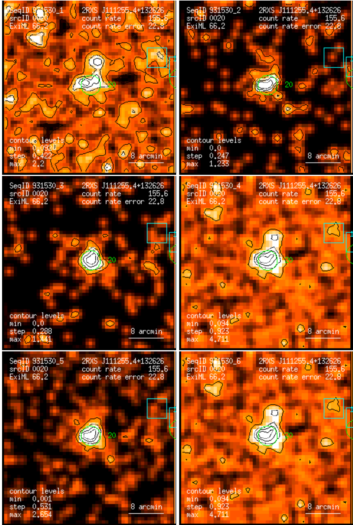
Figure 20: RASS 931530: detection 0020: band rate images, Gaussian filter: (1) PSPC channels 11 – 41, (2) 52 – 90, (3) 91 – 201, (4) 11 – 235, (5) 52 – 201, (6) 11 – 201. Broad band rates in counts/ks. Band rate contour levels in counts/ks/arcmin 2 .
