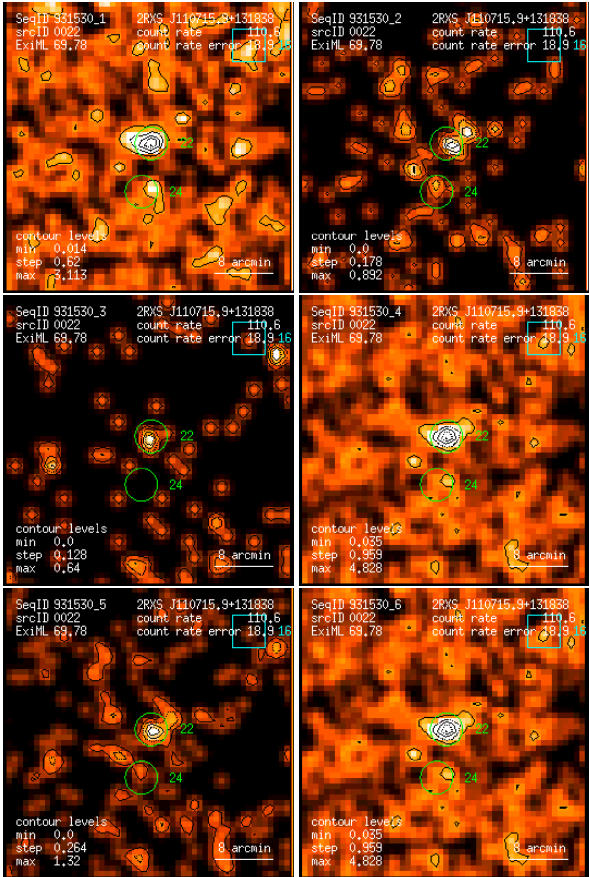
Figure 22: RASS 931530: detection 0022: band rate images, Gaussian filter: (1) PSPC channels 11 – 41, (2) 52 – 90, (3) 91 – 201, (4) 11 – 235, (5) 52 – 201, (6) 11 – 201. Broad band rates in counts/ks. Band rate contour levels in counts/ks/arcmin 2 .
