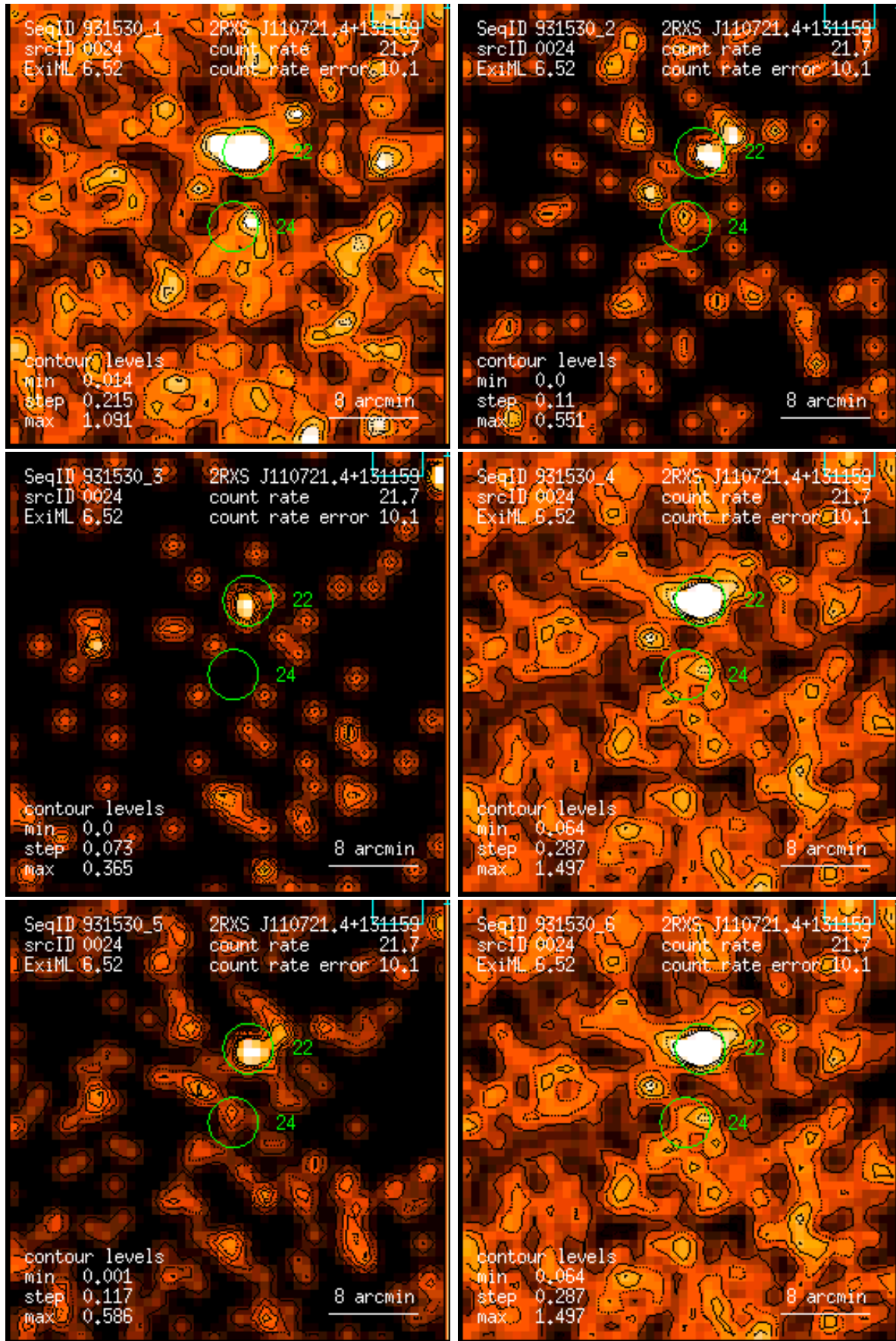
Figure 24: RASS 931530: detection 0024: band rate images, Gaussian filter: (1) PSPC channels 11 – 41, (2) 52 – 90, (3) 91 – 201, (4) 11 – 235, (5) 52 – 201, (6) 11 – 201. Broad band rates in counts/ks. Band rate contour levels in counts/ks/arcmin 2 .
