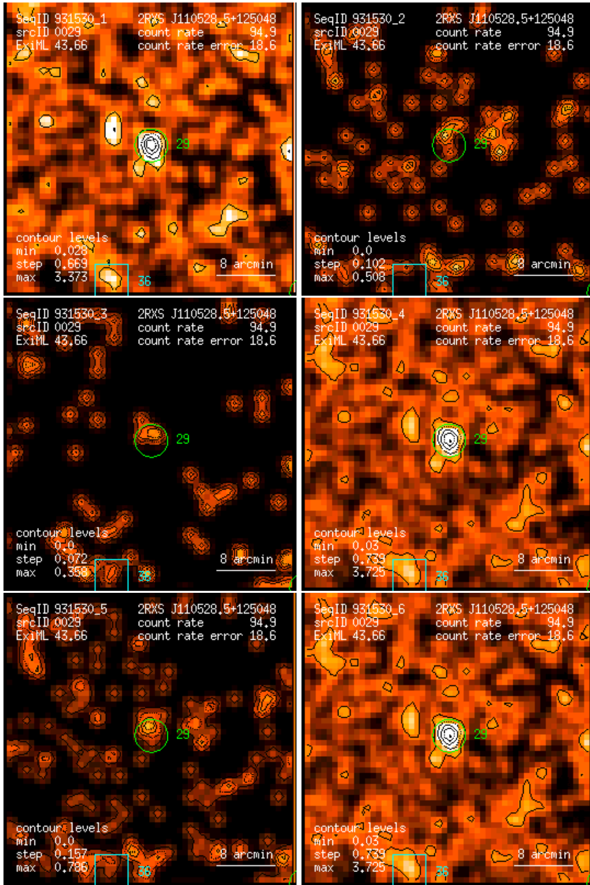
Figure 29: RASS 931530: detection 0029: band rate images, Gaussian filter: (1) PSPC channels 11 – 41, (2) 52 – 90, (3) 91 – 201, (4) 11 – 235, (5) 52 – 201, (6) 11 – 201. Broad band rates in counts/ks. Band rate contour levels in counts/ks/arcmin 2 .
