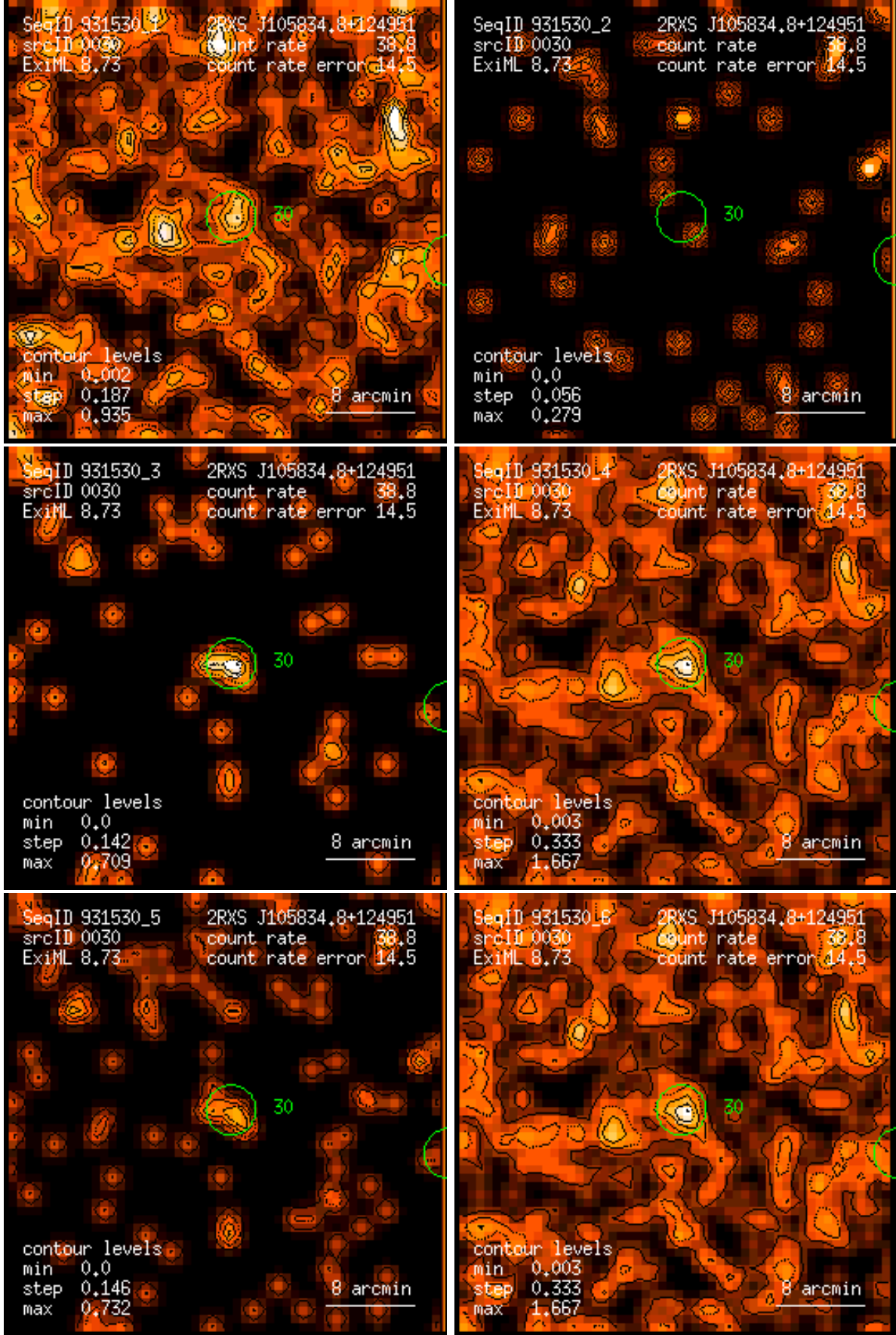
Figure 30: RASS 931530: detection 0030: band rate images, Gaussian filter: (1) PSPC channels 11 – 41, (2) 52 – 90, (3) 91 – 201, (4) 11 – 235, (5) 52 – 201, (6) 11 – 201. Broad band rates in counts/ks. Band rate contour levels in counts/ks/arcmin 2 .
