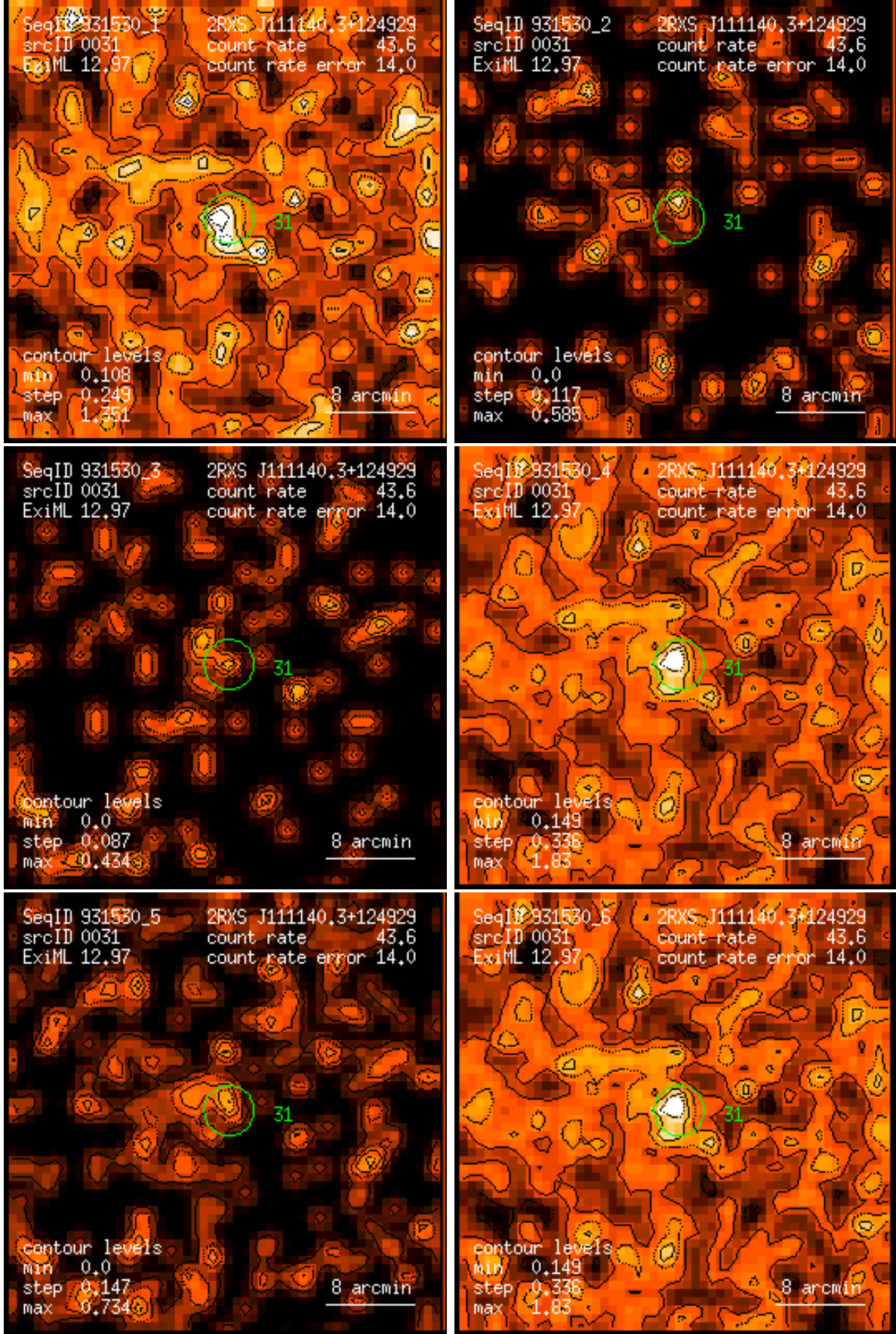
Figure 31: RASS 931530: detection 0031: band rate images, Gaussian filter: (1) PSPC channels 11 – 41, (2) 52 – 90, (3) 91 – 201, (4) 11 – 235, (5) 52 – 201, (6) 11 – 201. Broad band rates in counts/ks. Band rate contour levels in counts/ks/arcmin 2 .
