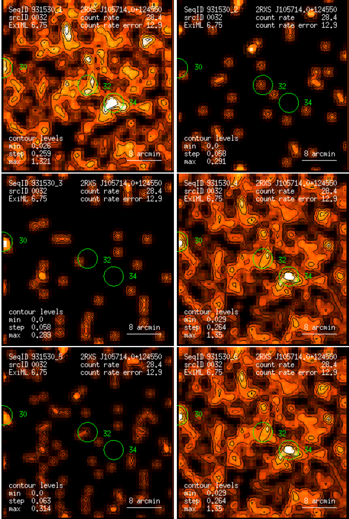
Figure 32: RASS 931530: detection 0032: band rate images, Gaussian filter: (1) PSPC channels 11 – 41, (2) 52 – 90, (3) 91 – 201, (4) 11 – 235, (5) 52 – 201, (6) 11 – 201. Broad band rates in counts/ks. Band rate contour levels in counts/ks/arcmin 2 .
