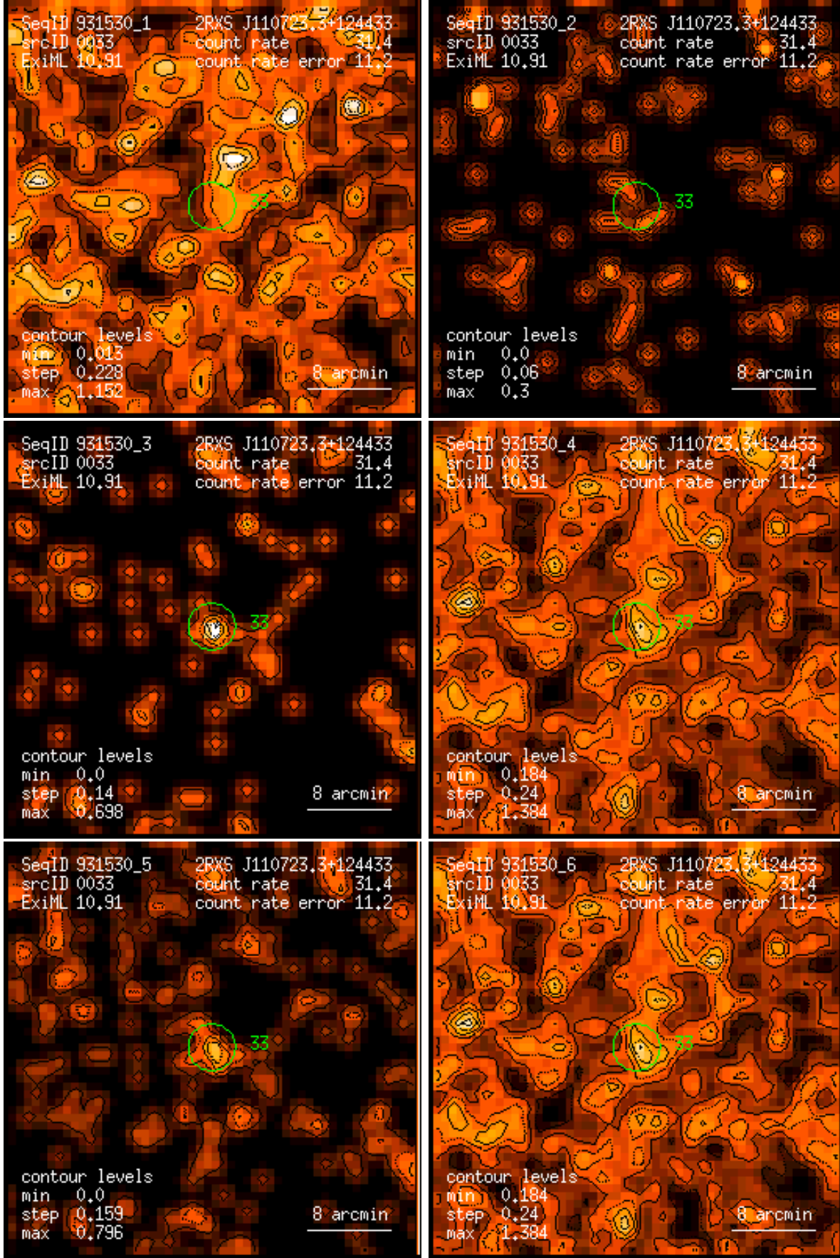
Figure 33: RASS 931530: detection 0033: band rate images, Gaussian filter: (1) PSPC channels 11 – 41, (2) 52 – 90, (3) 91 – 201, (4) 11 – 235, (5) 52 – 201, (6) 11 – 201. Broad band rates in counts/ks. Band rate contour levels in counts/ks/arcmin 2 .
