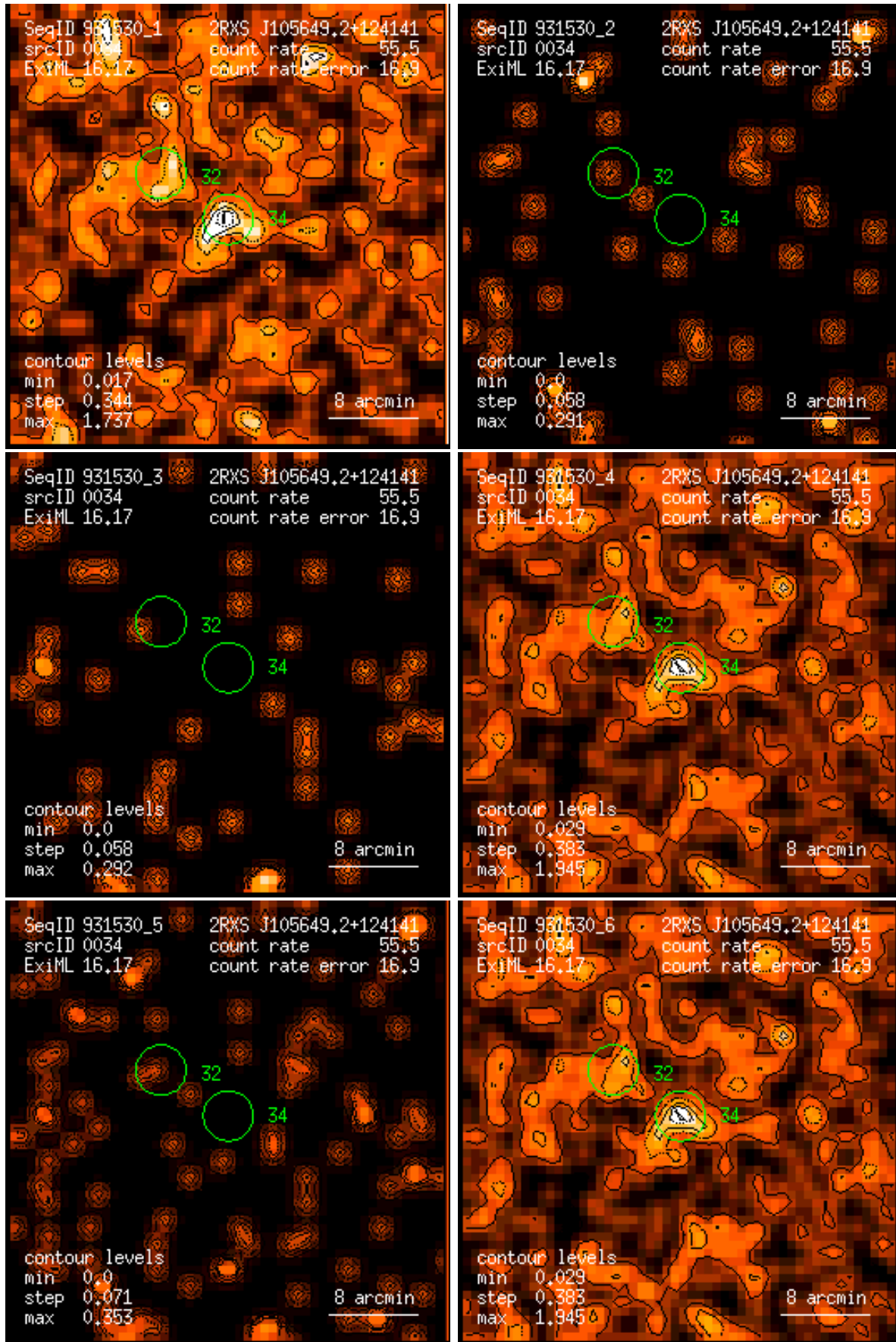
Figure 34: RASS 931530: detection 0034: band rate images, Gaussian filter: (1) PSPC channels 11 – 41, (2) 52 – 90, (3) 91 – 201, (4) 11 – 235, (5) 52 – 201, (6) 11 – 201. Broad band rates in counts/ks. Band rate contour levels in counts/ks/arcmin 2 .
