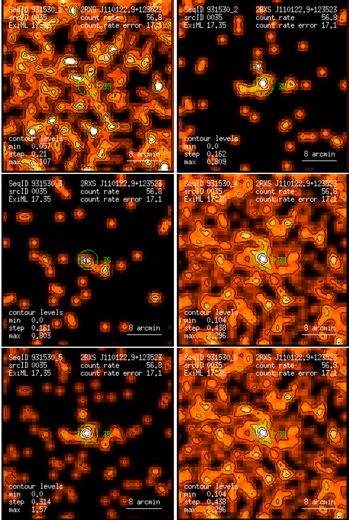
Figure 35: RASS 931530: detection 0035: band rate images, Gaussian filter: (1) PSPC channels 11 – 41, (2) 52 – 90, (3) 91 – 201, (4) 11 – 235, (5) 52 – 201, (6) 11 – 201. Broad band rates in counts/ks. Band rate contour levels in counts/ks/arcmin 2 .
