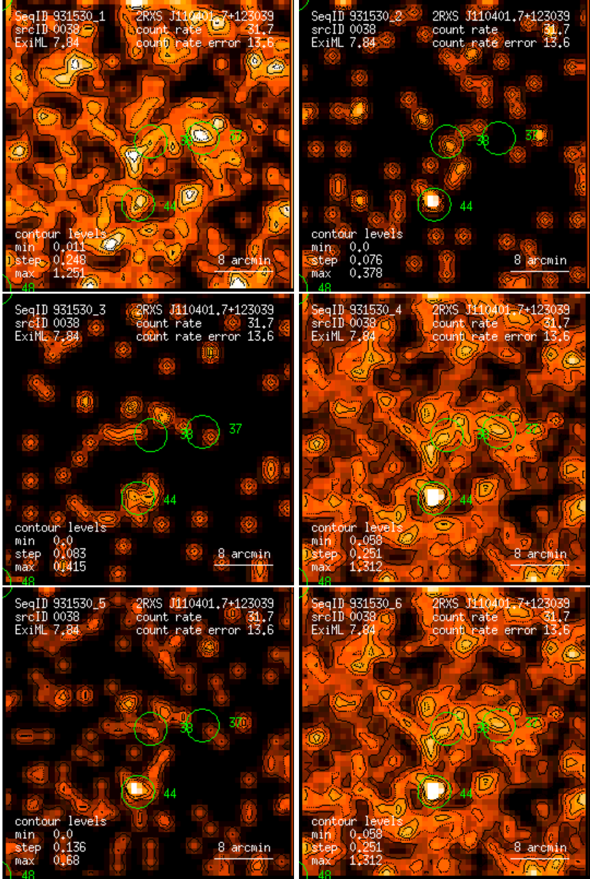
Figure 38: RASS 931530: detection 0038: band rate images, Gaussian filter: (1) PSPC channels 11 – 41, (2) 52 – 90, (3) 91 – 201, (4) 11 – 235, (5) 52 – 201, (6) 11 – 201. Broad band rates in counts/ks. Band rate contour levels in counts/ks/arcmin 2 .
