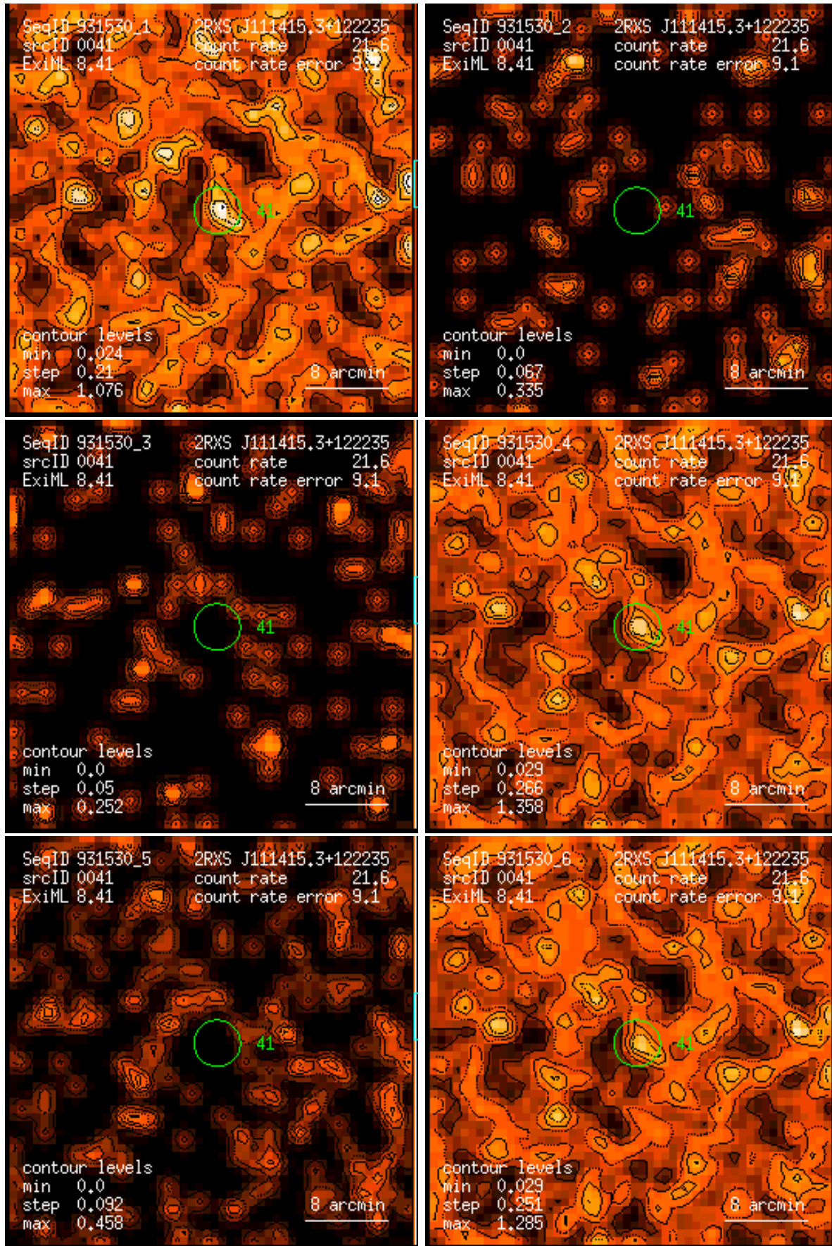
Figure 41: RASS 931530: detection 0041: band rate images, Gaussian filter: (1) PSPC channels 11 – 41, (2) 52 – 90, (3) 91 – 201, (4) 11 – 235, (5) 52 – 201, (6) 11 – 201. Broad band rates in counts/ks. Band rate contour levels in counts/ks/arcmin 2 .
