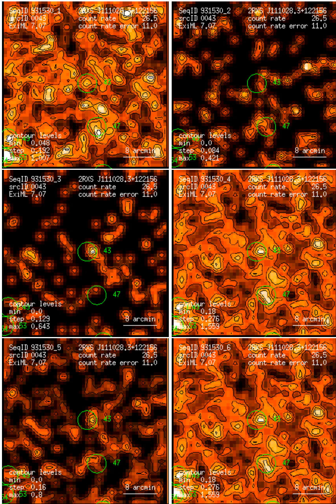
Figure 43: RASS 931530: detection 0043: band rate images, Gaussian filter: (1) PSPC channels 11 – 41, (2) 52 – 90, (3) 91 – 201, (4) 11 – 235, (5) 52 – 201, (6) 11 – 201. Broad band rates in counts/ks. Band rate contour levels in counts/ks/arcmin 2 .
