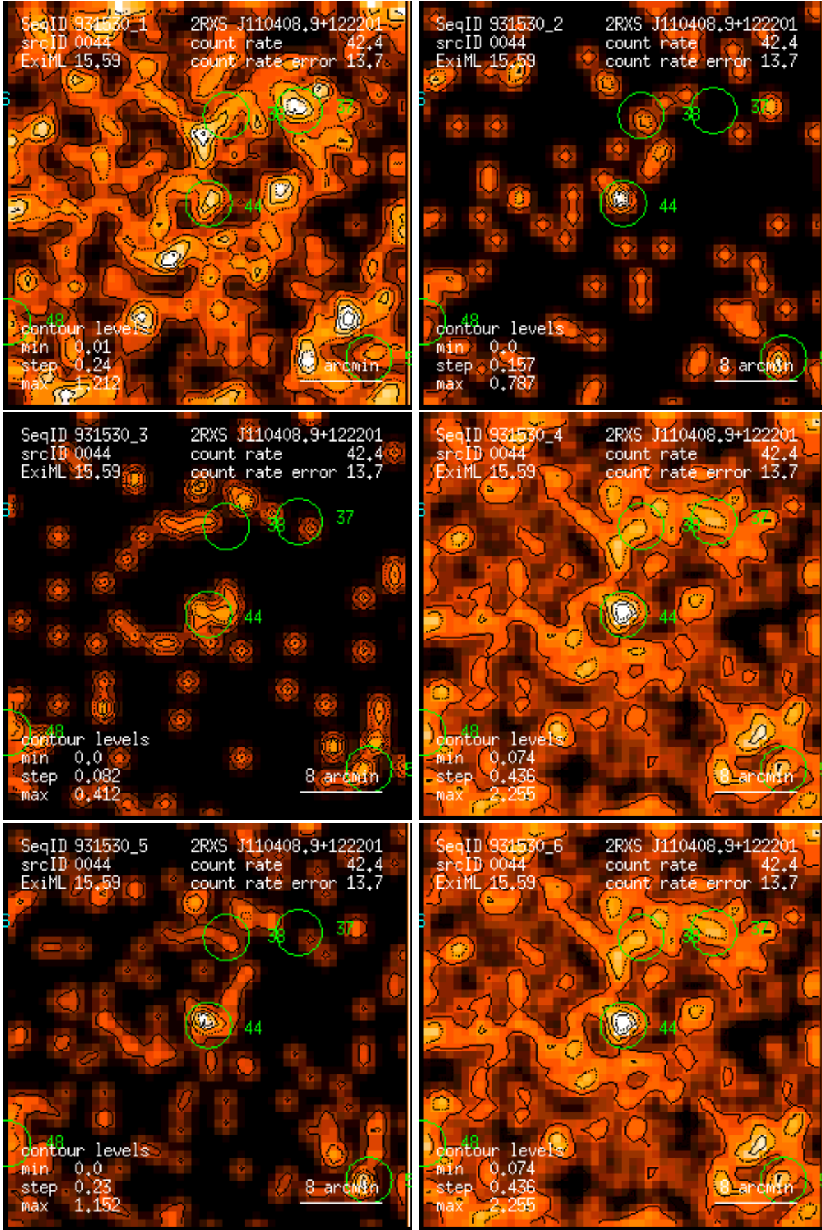
Figure 44: RASS 931530: detection 0044: band rate images, Gaussian filter: (1) PSPC channels 11 – 41, (2) 52 – 90, (3) 91 – 201, (4) 11 – 235, (5) 52 – 201, (6) 11 – 201. Broad band rates in counts/ks. Band rate contour levels in counts/ks/arcmin 2 .
